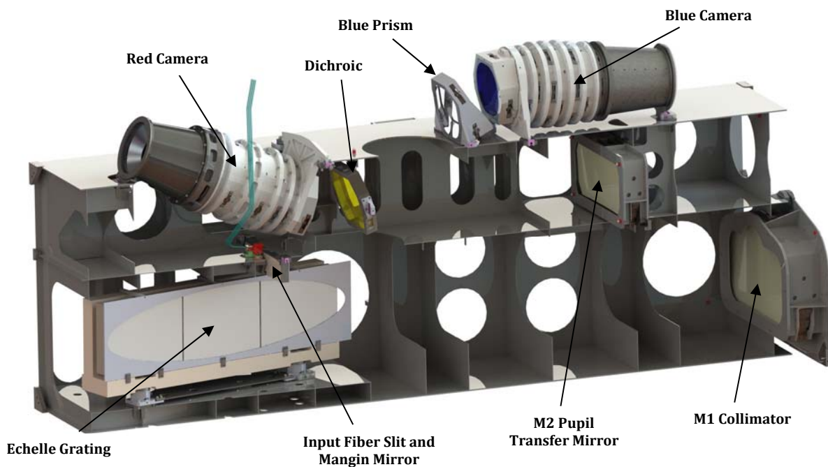
Figure 7 – Bench Sectioned
