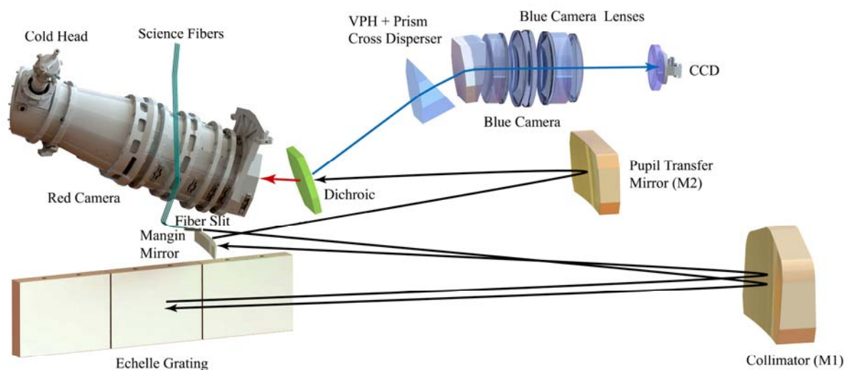
Figure 2 - Spectrograph Optical Layout
