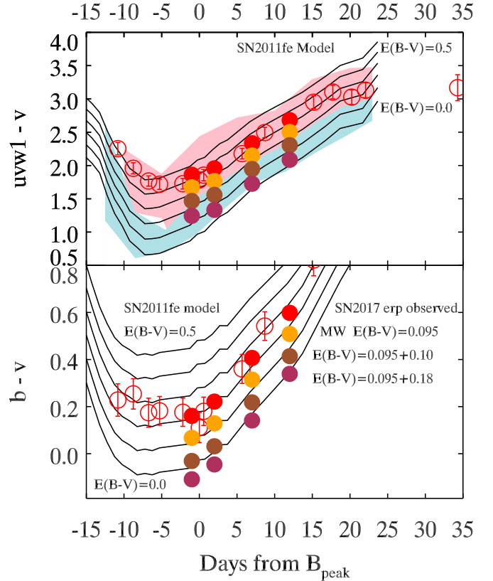
Figure 6. Observed and reddening-corrected uvw1 - v and b - v color evolutions of SN 2017erp are compared with regions occupied by SNe Ia identified as NUV-red (pink shaded region) and NUV-blue (blue shaded region) by Milne et al. (2013) and a spectroscopic model of SN 2011fe (Pereira et al. 2013) with different amounts of reddening applied (represented by solid curves). The photometric observations of SN 2017erp are indicated by open circles. Filled circles show the spectrophotometric colors from the HST observations of SN 2017erp with various amounts of reddening applied (the same color circles are used in both panels and labeled in the bottom panel). For the largest amount of reddening, SN 2017erp has colors most similar to the NUV-blue group, but the B - V color is also bluer than the SN 2011fe template.
