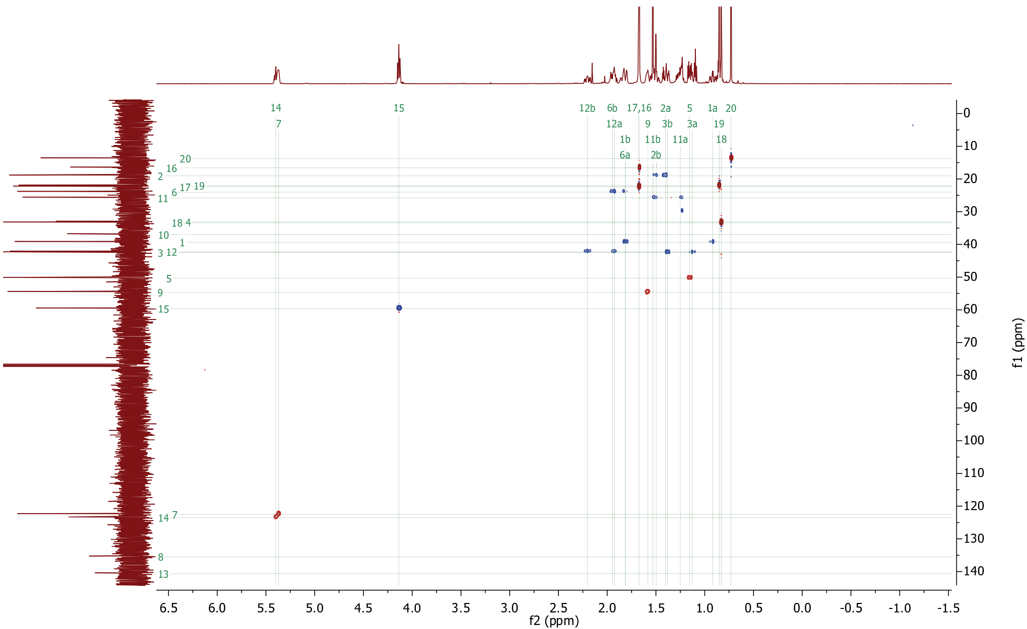
Figure S11-D. ^1\text{H} - ^{13}\text{C} HSQC of labda-7,13E-dien-15-ol [21a]
