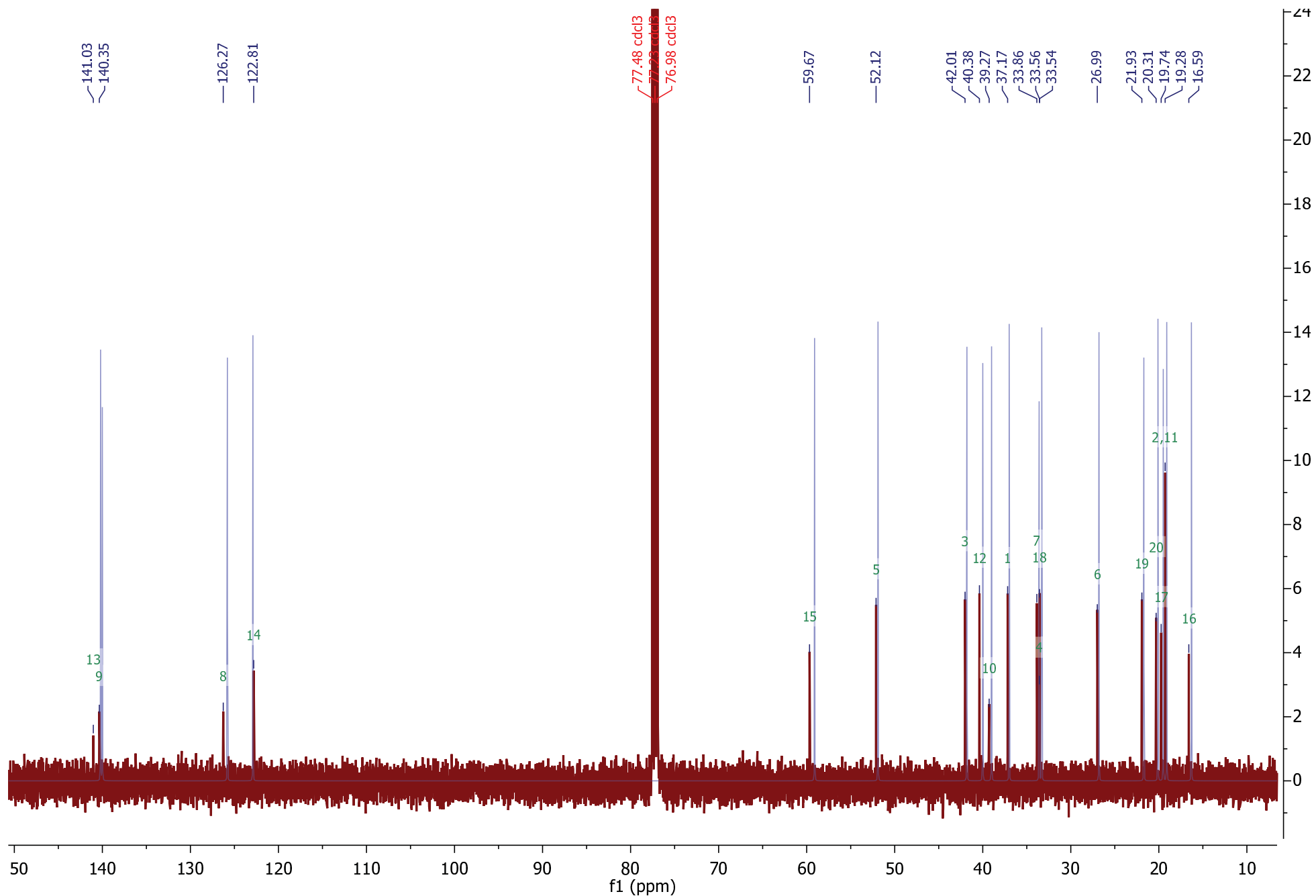
Figure S14-G. Overlay of ^{13}\text{C} NMR of (10R)-labda-8,13E-diene-15-ol [25a] (red) with ^{13}\text{C} NMR spectrum (blue) reconstructed from shifts reported for the same compound by Suzuki et al. (1983) (DOI: 10.1016/0031-9422(83)80249-0).
