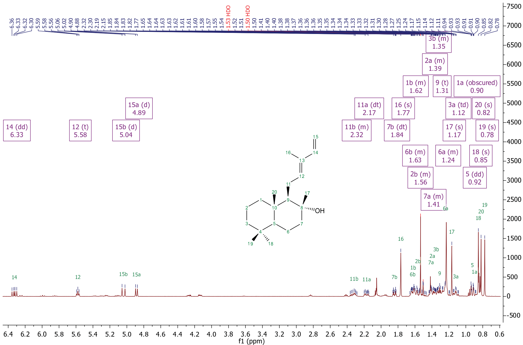
Figure S10-A. ^1\text{H} NMR of trans-abienol [11].
