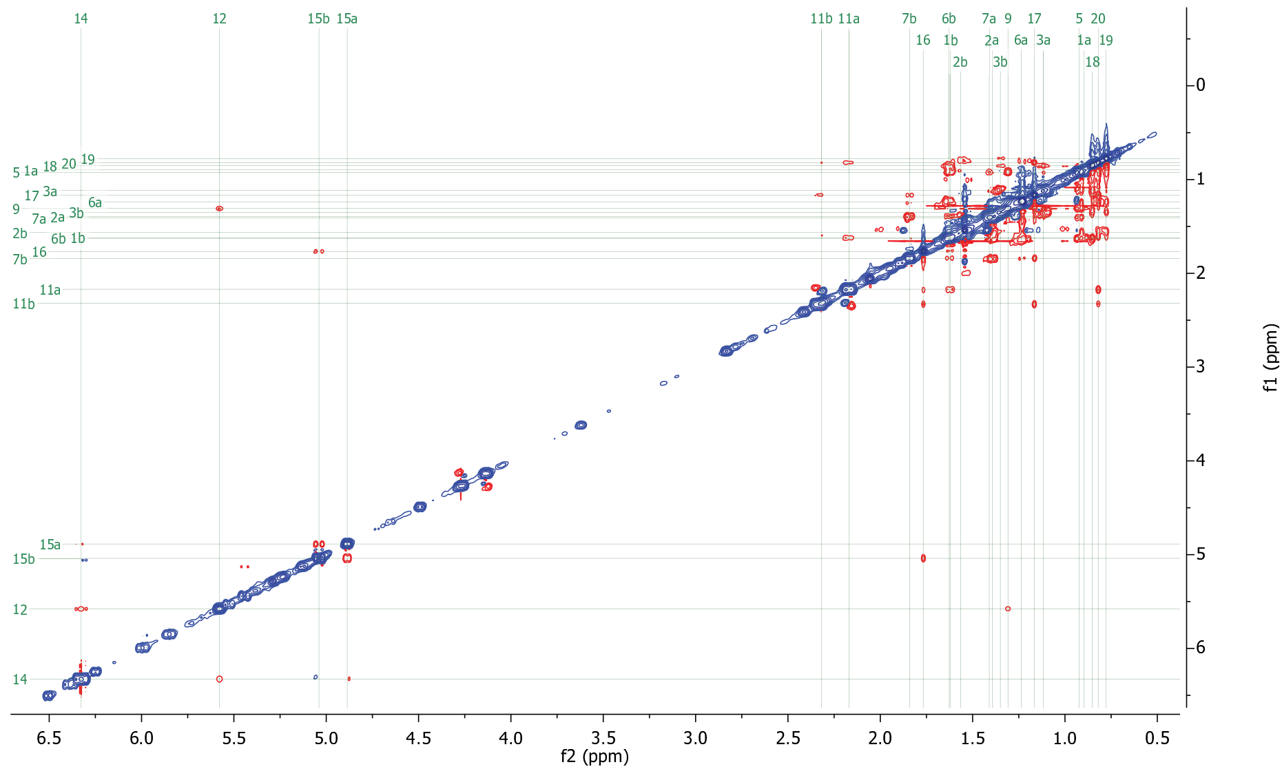
Figure S10-F. ^1\text{H} NOESY of trans-abienol [11].
