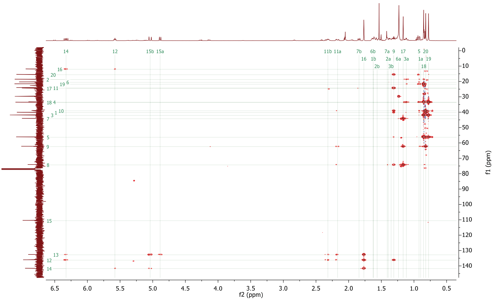
Figure S10-E. ^1\text{H} - ^{13}\text{C} HMBC of trans-abienol [11].
