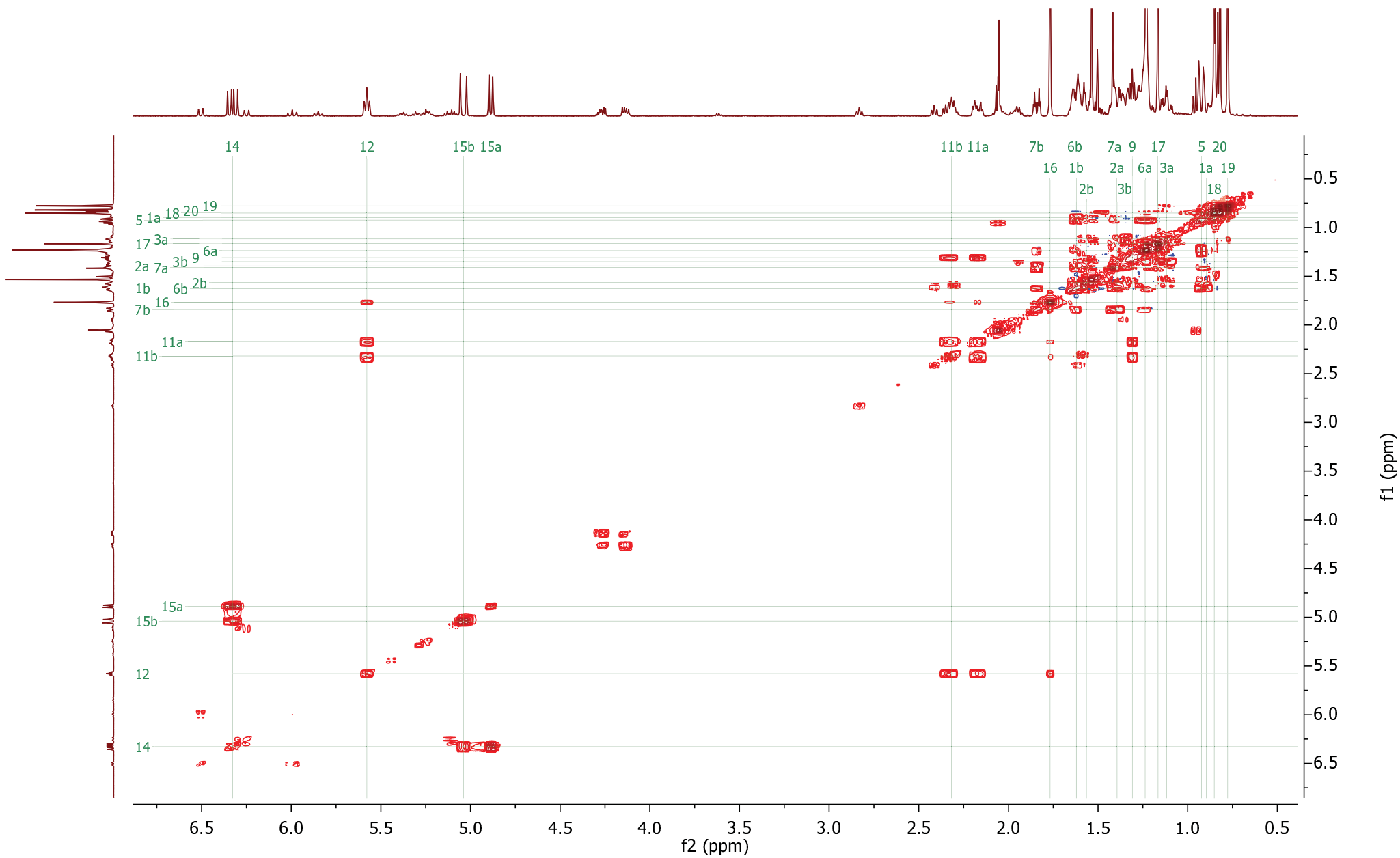
Figure S10-C. 1 H- 1 H COSY of trans-abienol [11].
