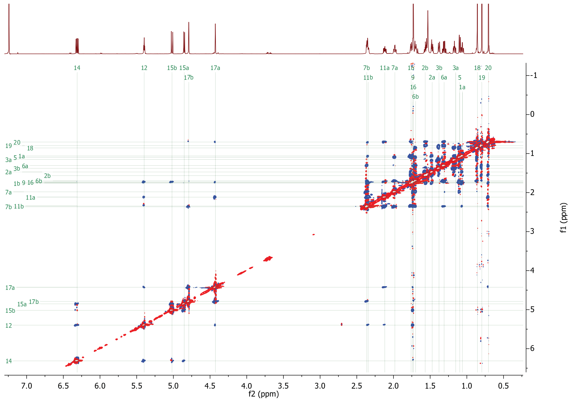
Figure S16-F. ^1\text{H} NOESY of trans-biformene [34].
