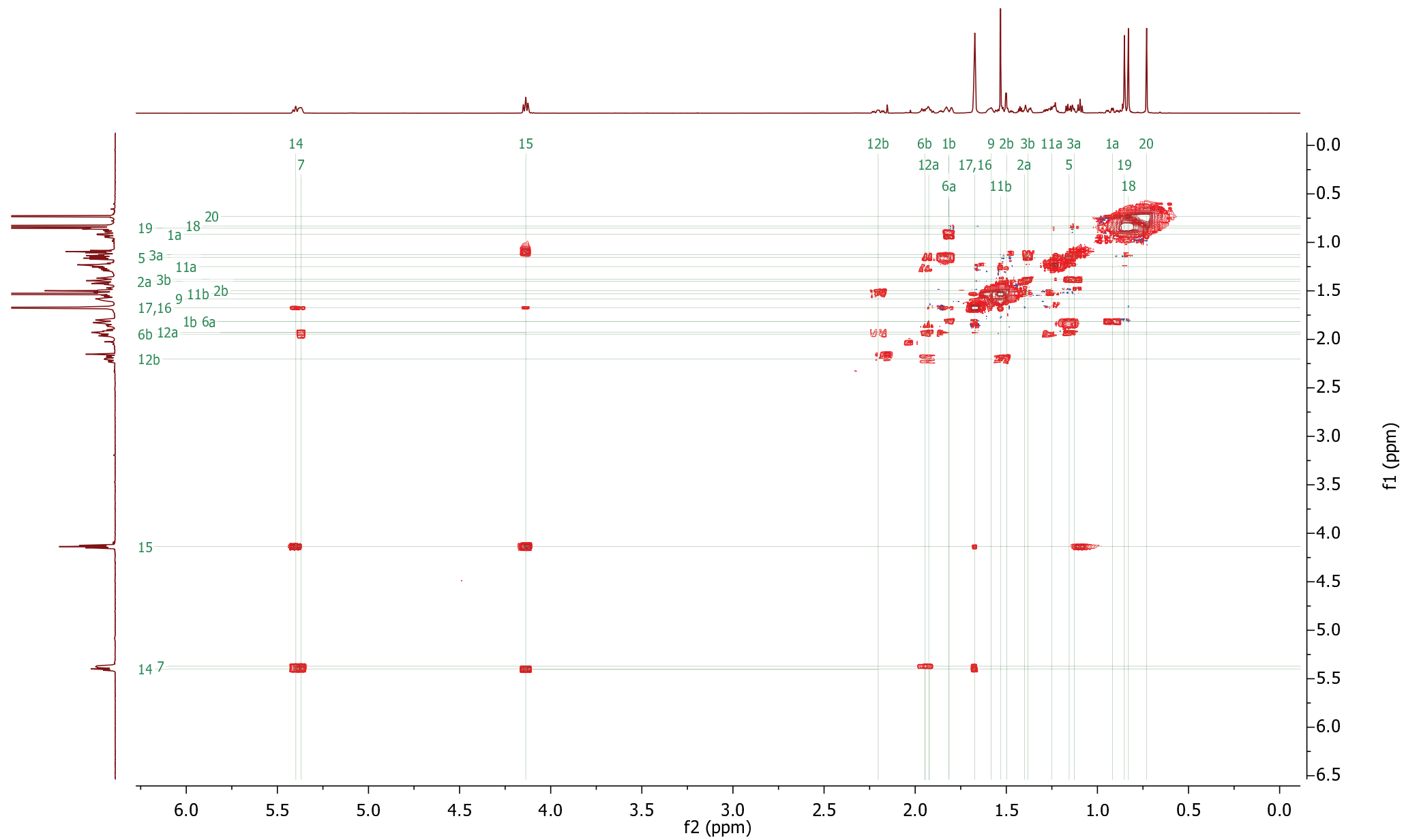
Figure S11-C. ^1\text{H} - ^1\text{H} COSY of \lambda -7,13E-dien-15-ol [21a].
