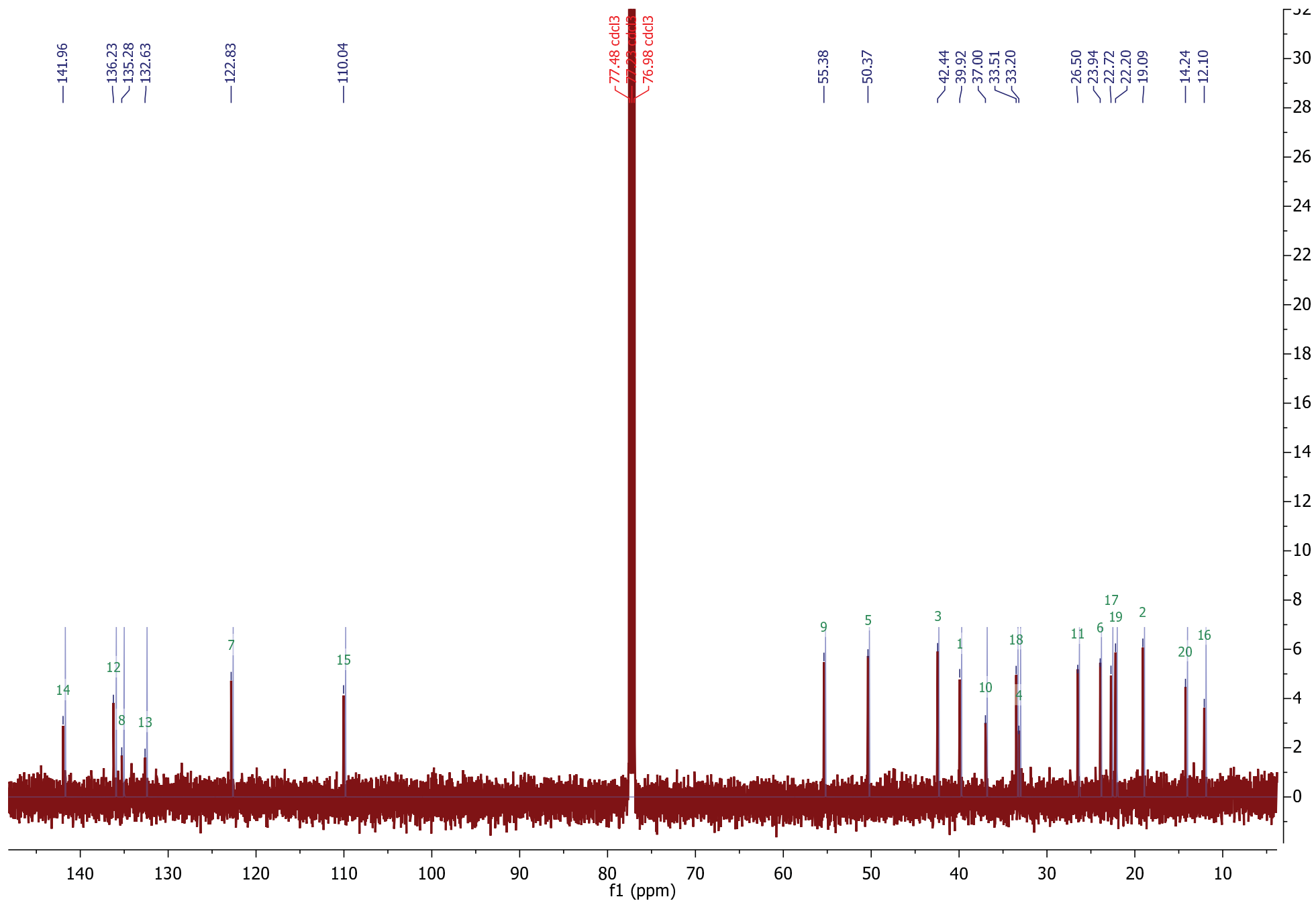
Figure S13-G. Overlay of ^{13}\text{C} NMR of labda-7,12E,14-triene [ 24 ] (red) with ^{13}\text{C} NMR spectrum (blue) reconstructed from shifts reported for the same compound by Roengsumran et al. (1999) (DOI: 10.1016/S0031-9422(98)00604-9).
