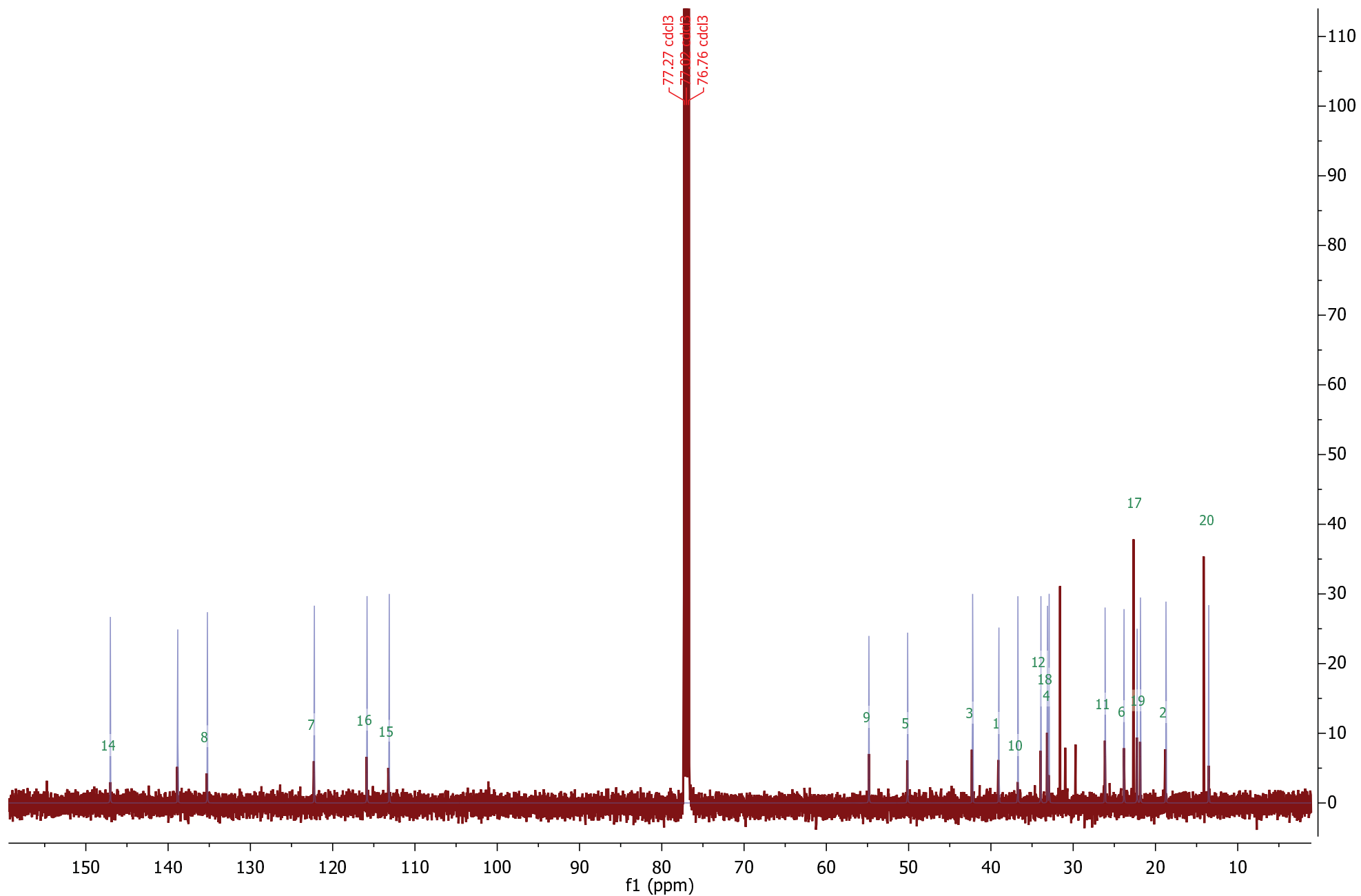
Figure S12-C. Overlay of ^{13}\text{C} NMR of partially purified labda-7,13(16),14-triene [22] (red) with ^{13}\text{C} NMR spectrum (blue) reconstructed from shifts reported for the same compound by Jia et al. (2016) (DOI: 10.1016/j.ymben.2016.04.001).
