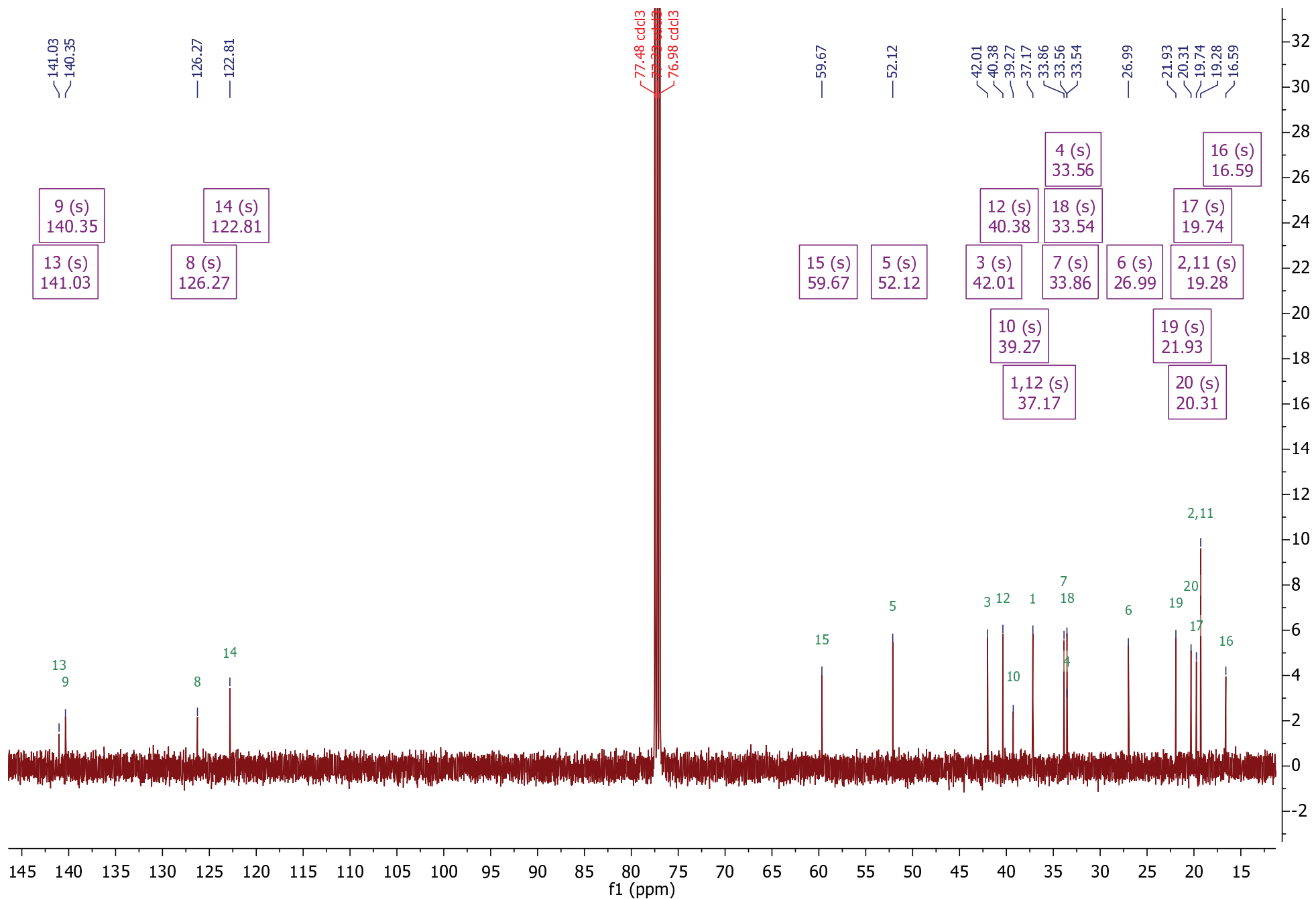
Figure S14-B. ^{13}\text{C} NMR of (10R)-labda-8,13E-diene-15-ol [25a].
