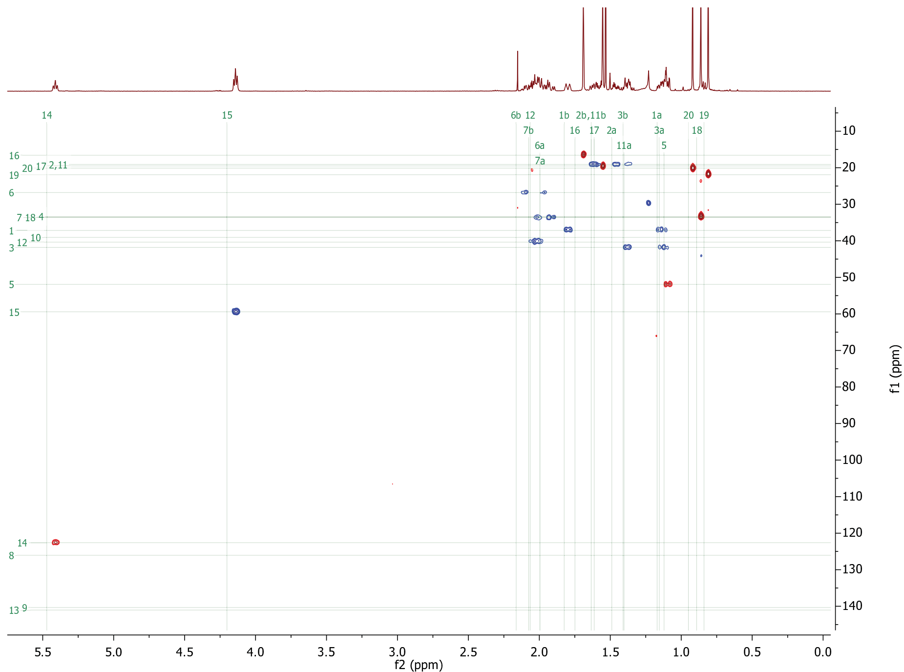
Figure S14-D. ^1\text{H} - ^{13}\text{C} HSQC of (10R)-labda-8,13E-diene-15-ol [ 25a ].
