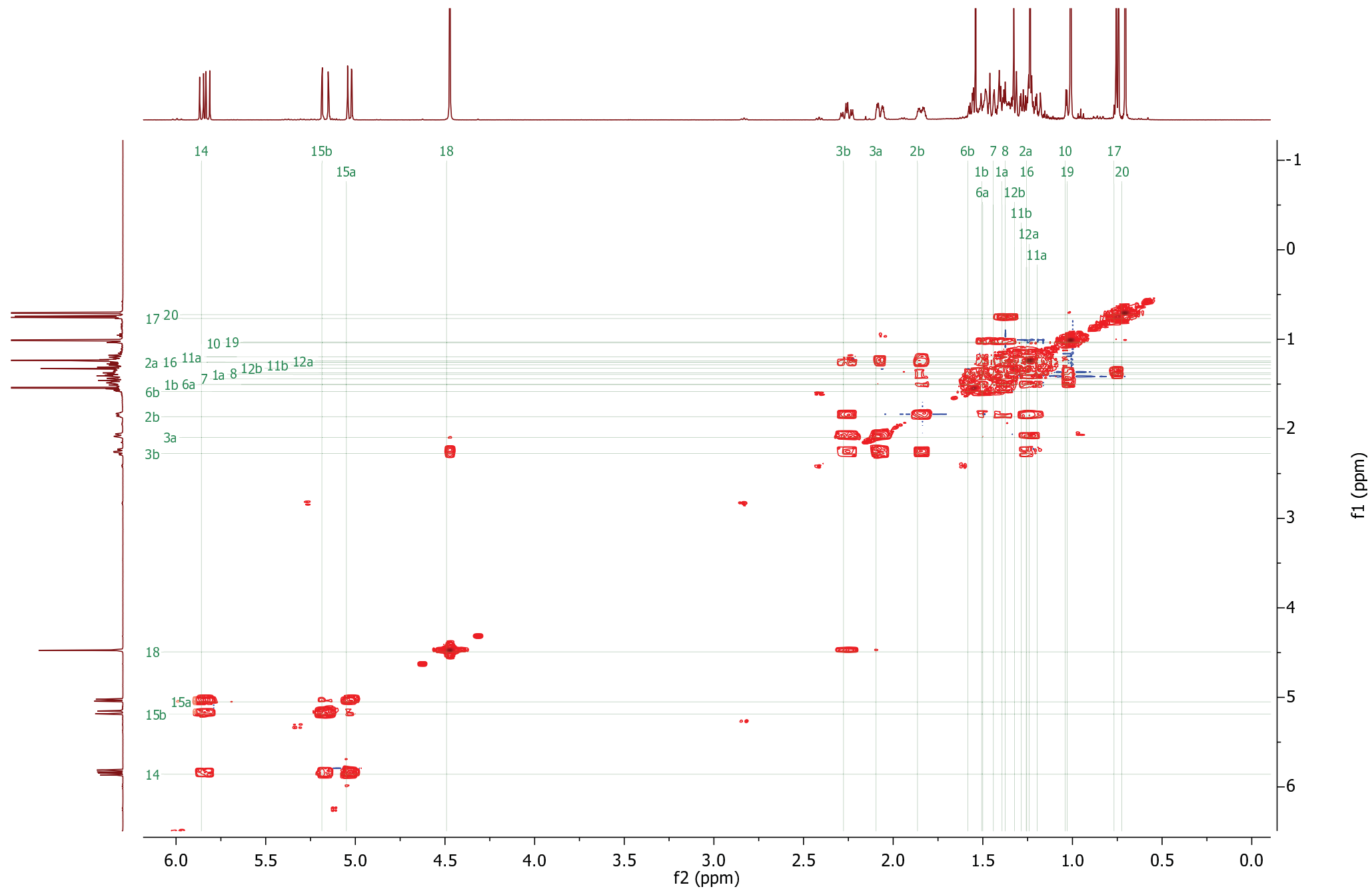
Figure S17-C. 1 H- 1 H COSY of neo-cleroda-4(18),14-dien-13-ol [37].
