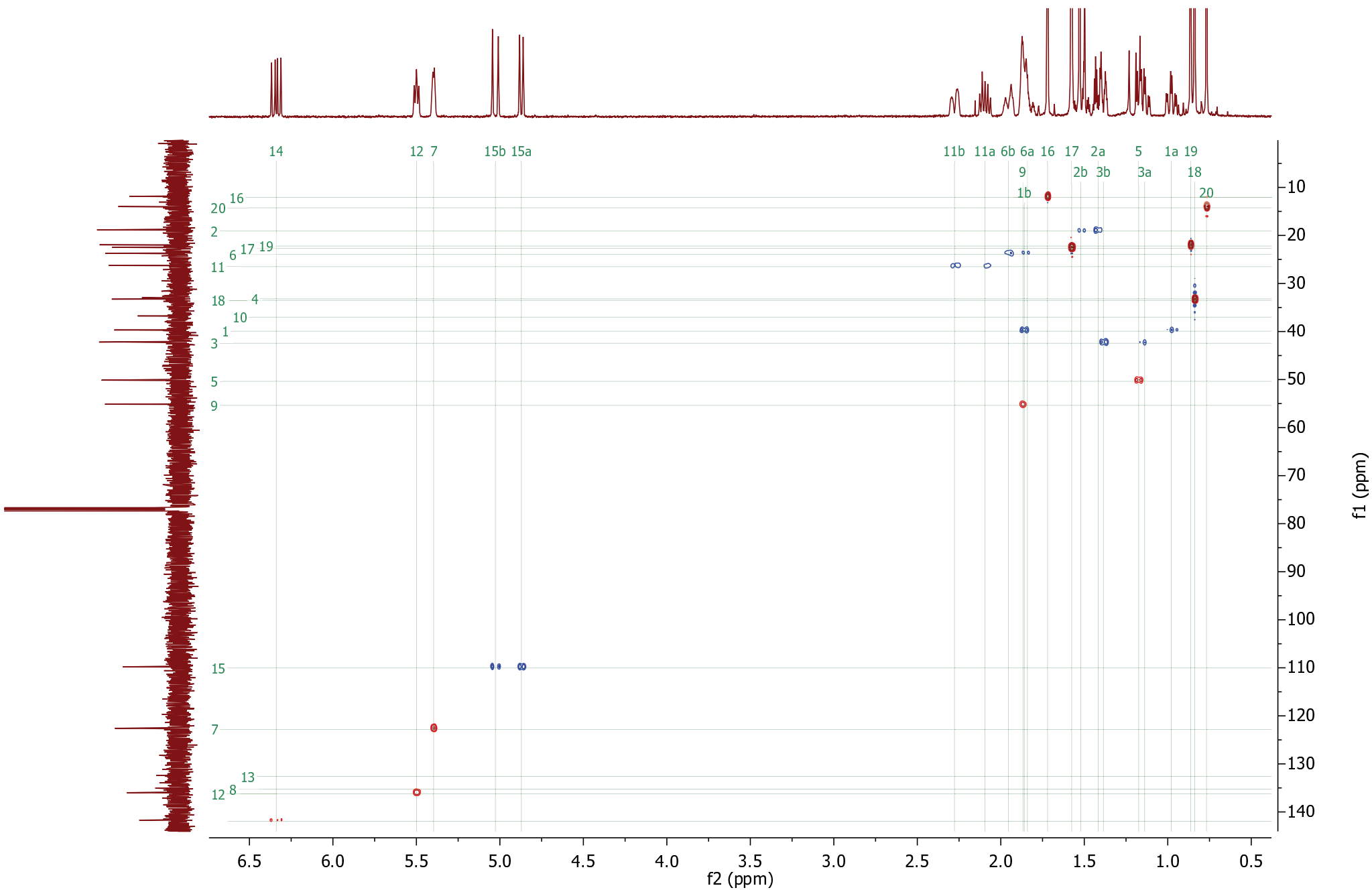
Figure S13-D. ^1\text{H} - ^{13}\text{C} HSQC of labda-7,12E,14-triene [24].
