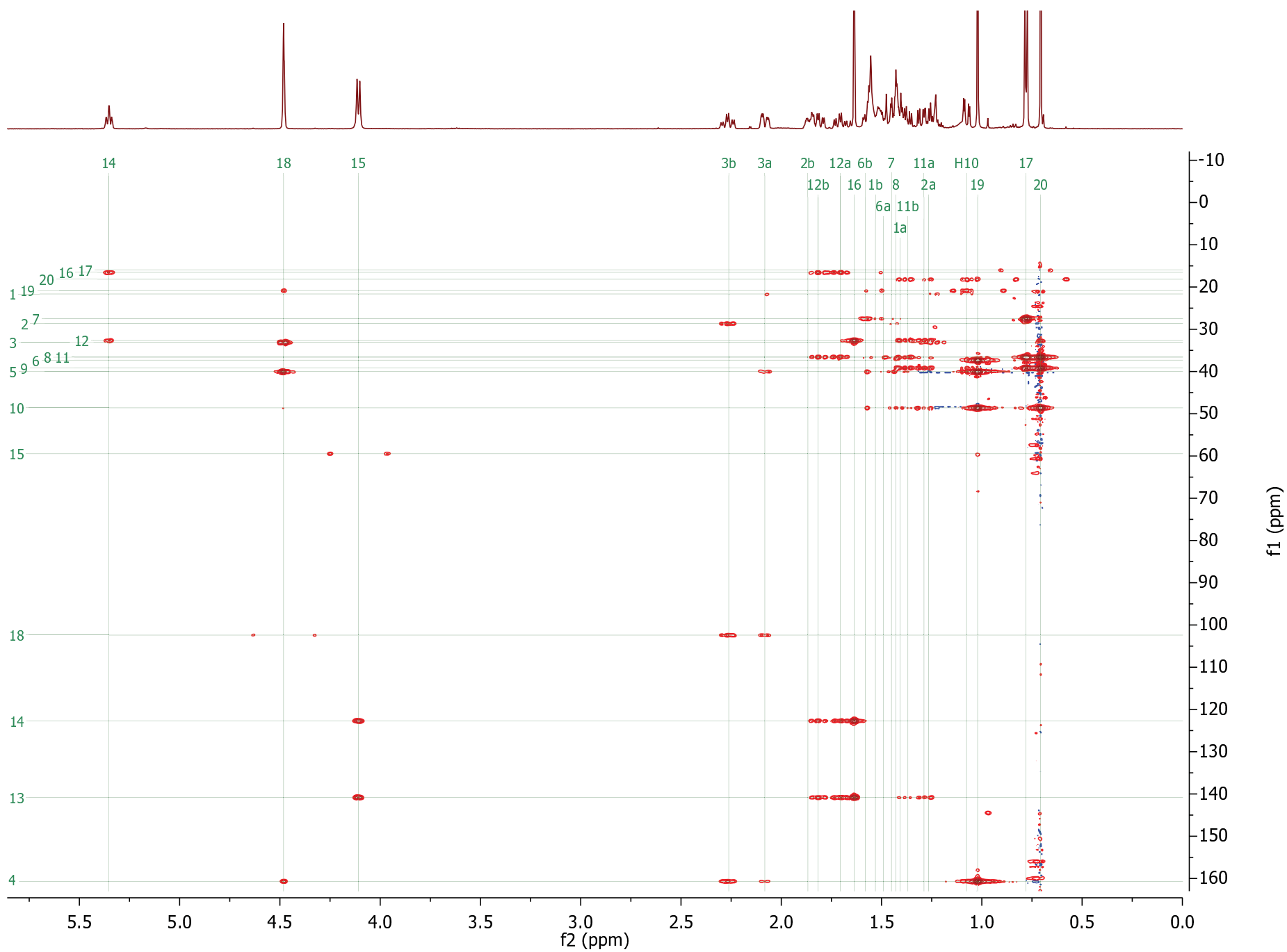
Figure S18-E. ^1\text{H} - ^{13}\text{C} HMBC of neo-cleroda-4(18),13E-diene-15-ol [38a].
