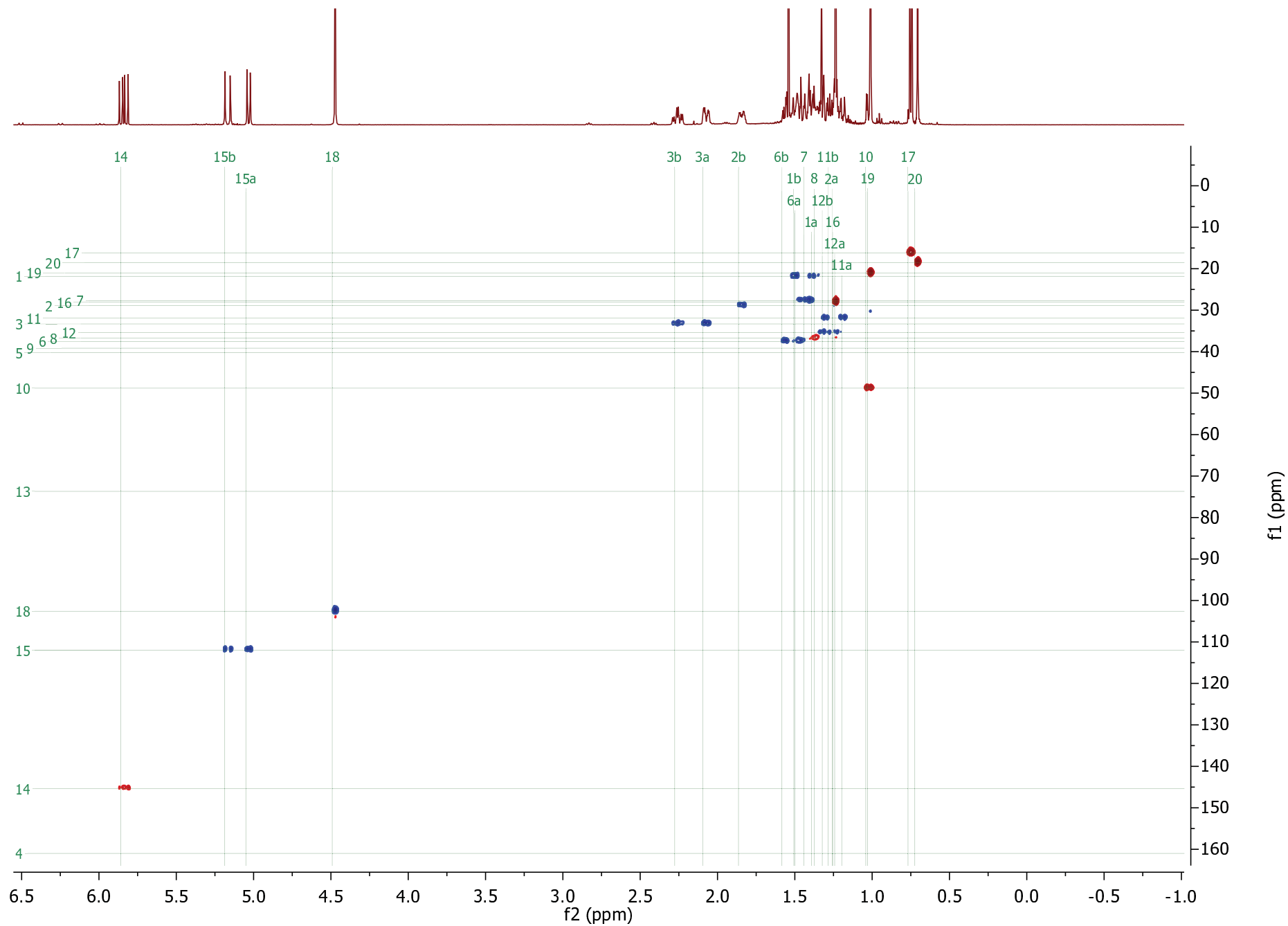
Figure S17-D. ^1\text{H} - ^{13}\text{C} HSQC of neo-cleroda-4(18),14-dien-13-ol [37].
