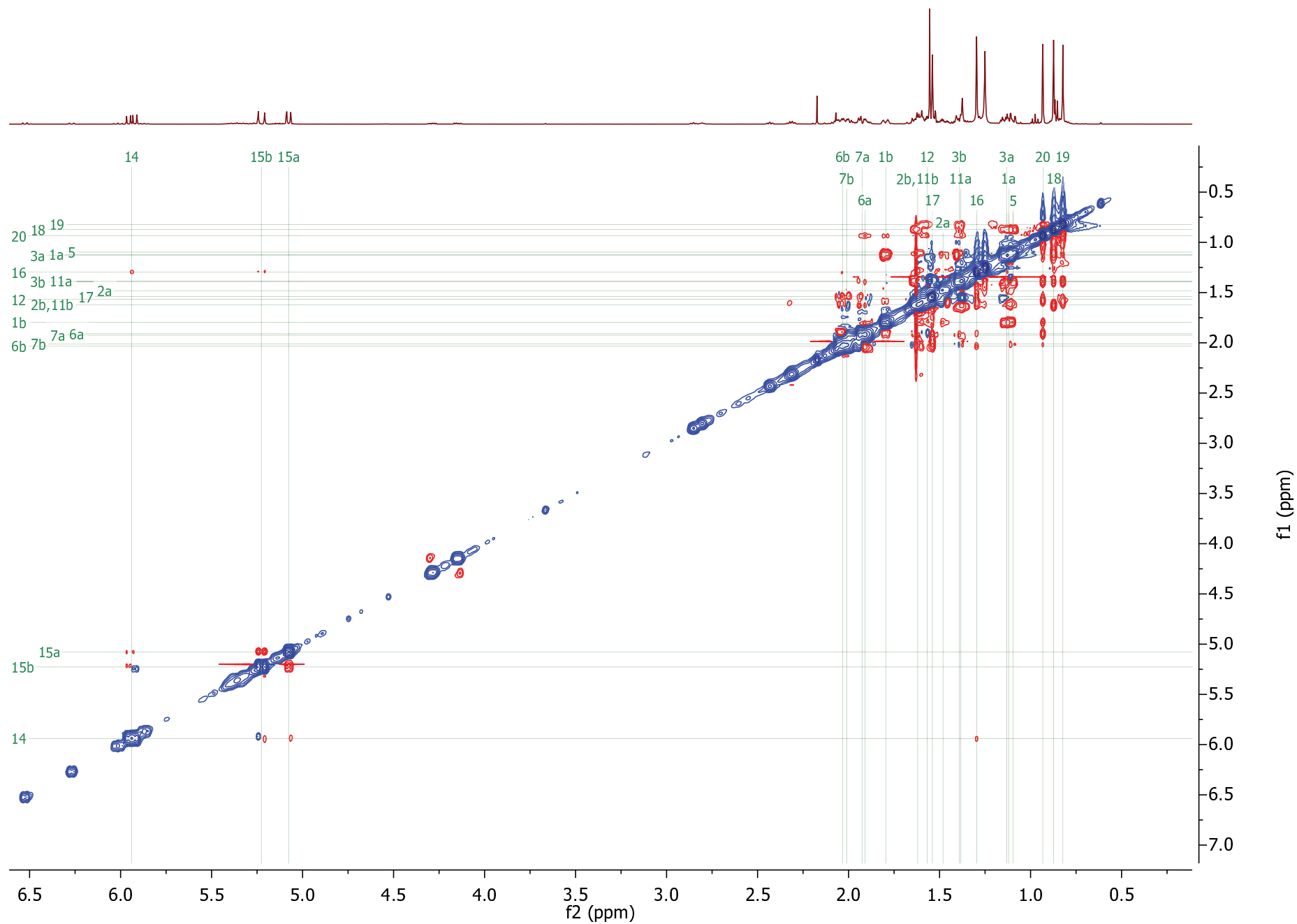
Figure S15-F. ^1\text{H} NOESY of (10R)-labda-8,14-dien-13-ol [26].
