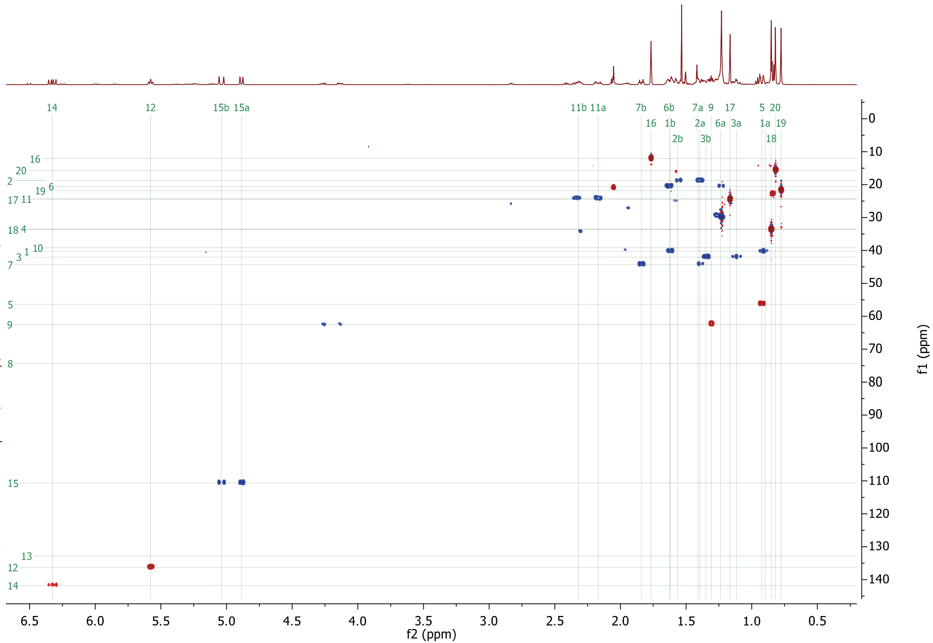
Figure S10-D. ^1\text{H} - ^{13}\text{C} HSQC of trans-abienol [11].
