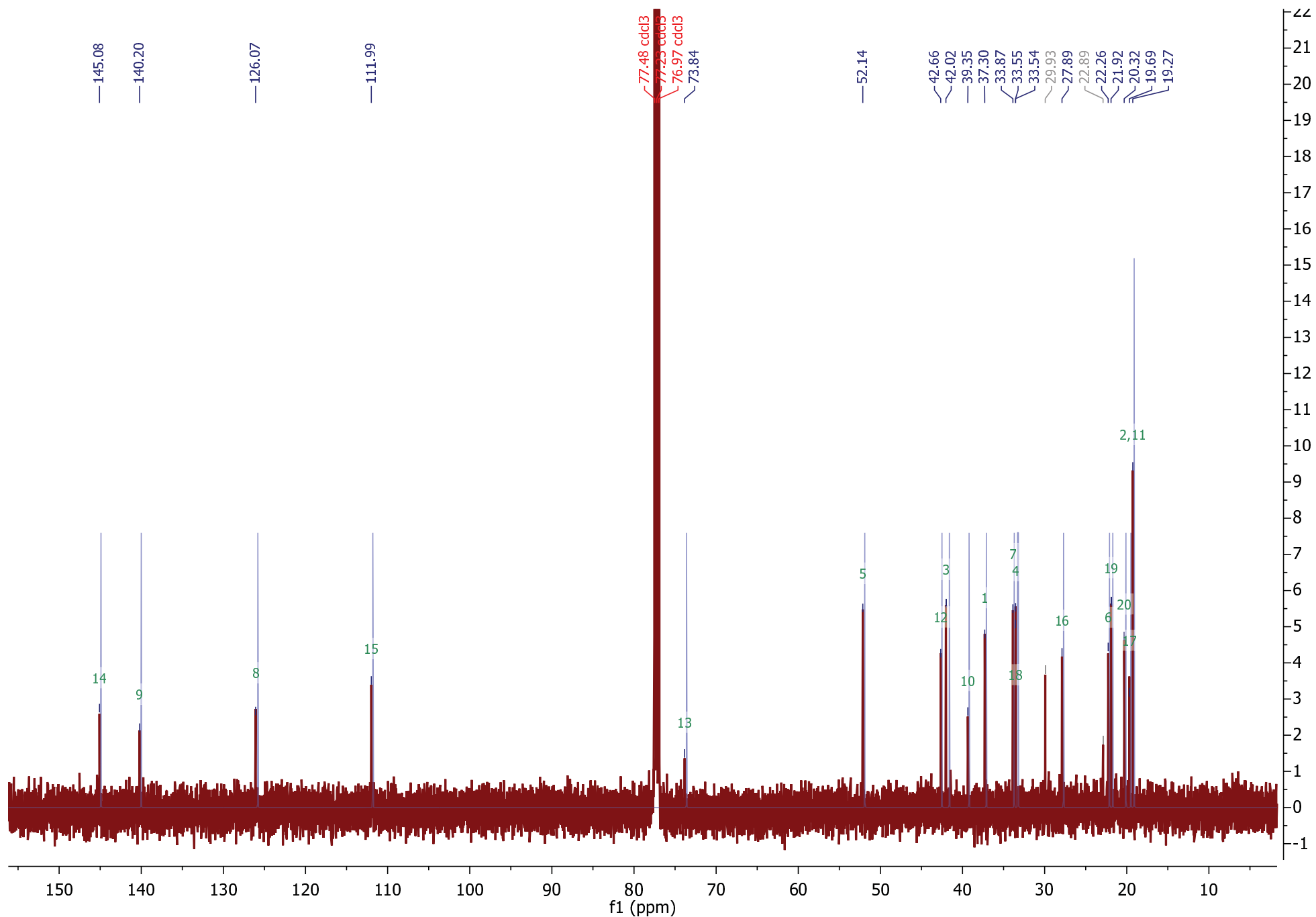
Figure S15-G. Overlay of ^{13}\text{C} NMR of (10R)-labda-8,14-dien-13-ol [26] (red) with ^{13}\text{C} NMR spectrum (blue) reconstructed from shifts reported for the same compound by Wu and Lin (1997) (DOI: 10.1016/S0031-9422(96)00519-5).
