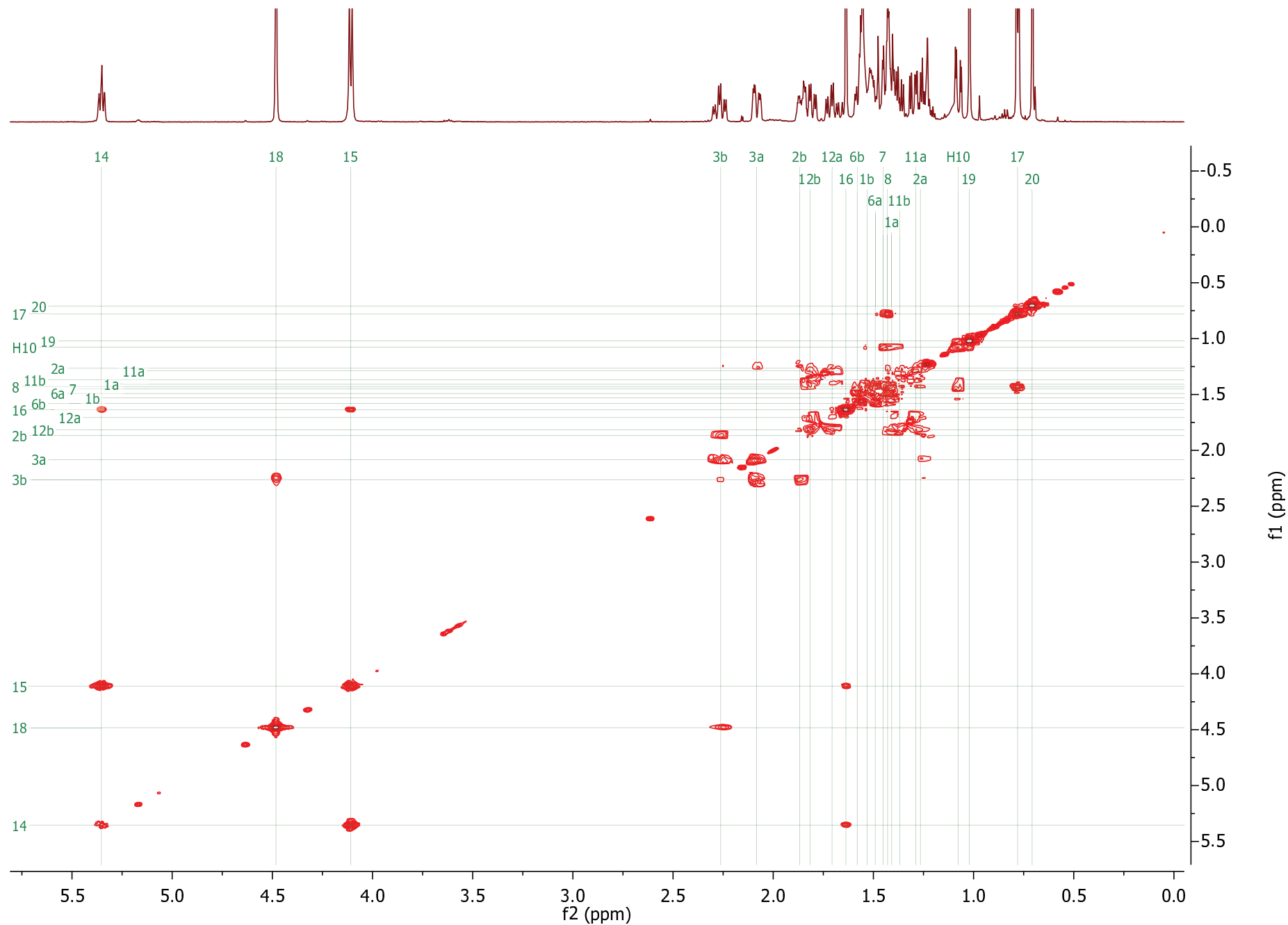
Figure S18-C. ^1\text{H} - ^1\text{H} COSY of neo-cleroda-4(18),13E-diene-15-ol [38a].
