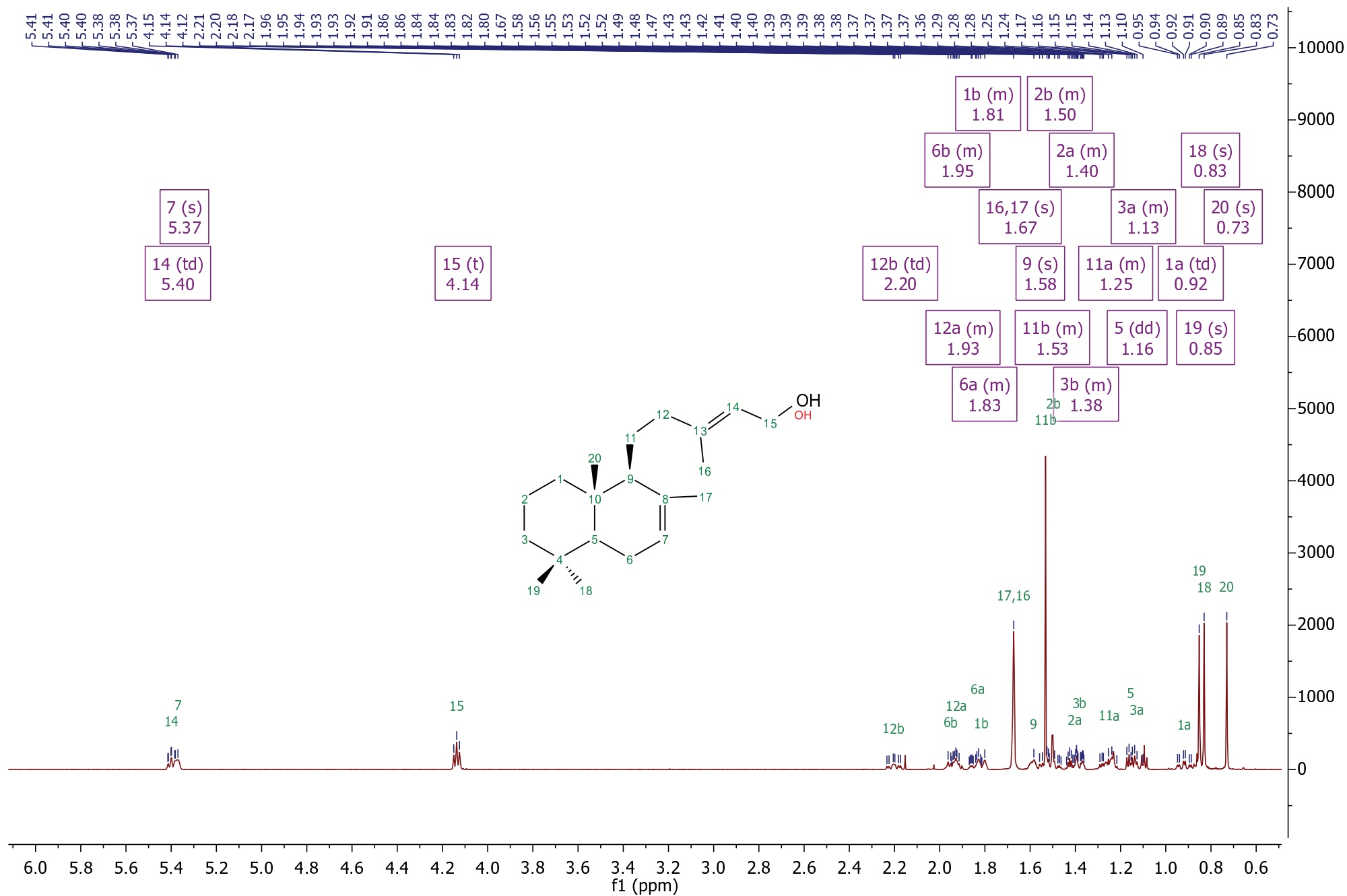
Figure S11-A. ^1\text{H} NMR of labda-7,13E-dien-15-ol [21a].
