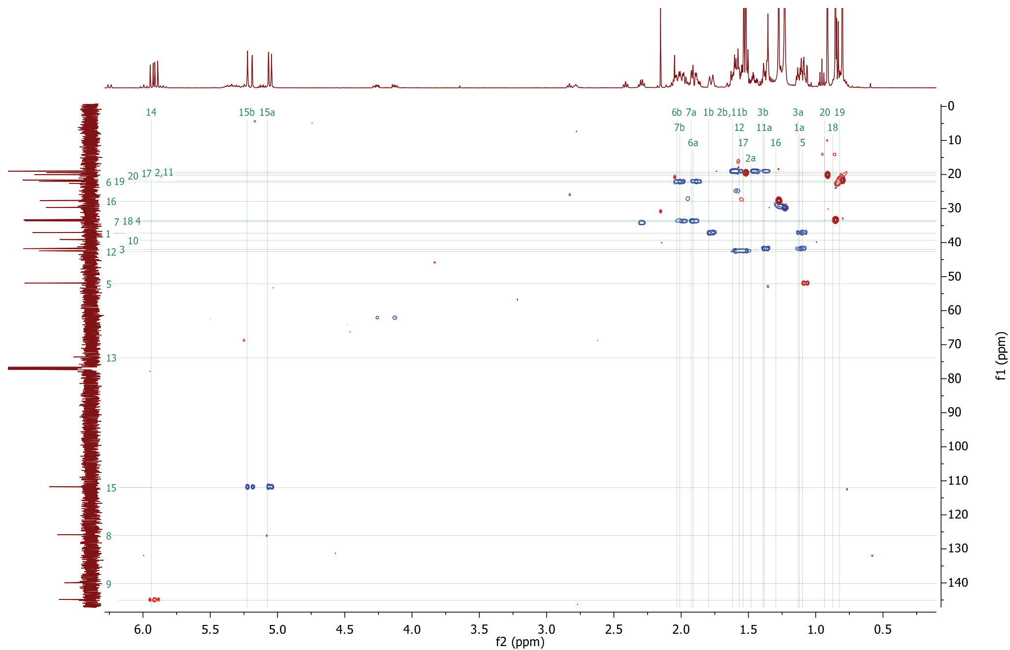
Figure S15-D. ^1\text{H} - ^{13}\text{C} HSQC of (10R)-labda-8,14-dien-13-ol [26].
