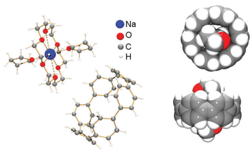
Fig. 2 Molecular structure of 2 (left, ball-and-stick model; THF inside the cavity of [6]CPP has been removed for clarity). Space-filling models of encapsulated THF molecules inside [6]CPP 1− (right).
