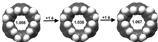
Fig. 4 Core transformation of 1 upon the addition of one and two electrons, space-filling models of [6]CPP, [6]CPP 1– , and [6]CPP 2– .
