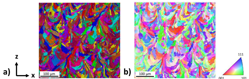
Fig. 4 EBSD maps showing a unique grain map and b inverse pole figure
