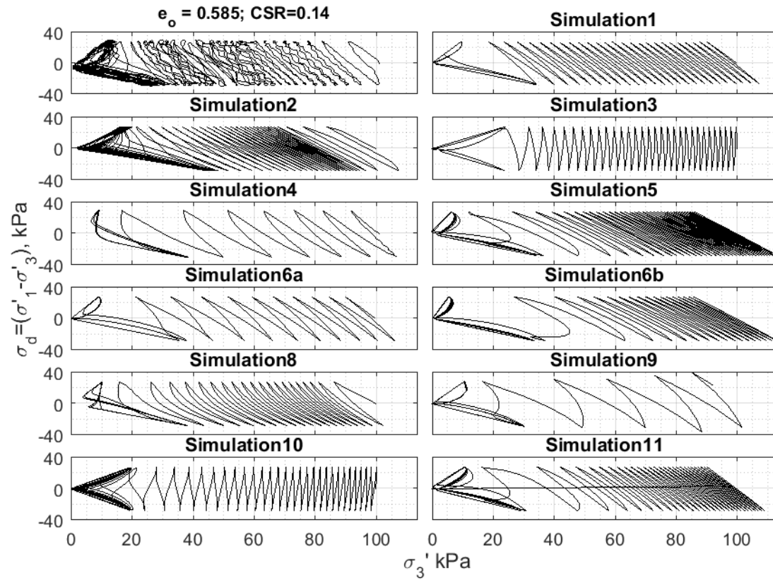
Figure 1-a. Comparison of the numerical simulations of stress paths for a cyclic stress-controlled test on Ottawa F65 sand. e = 0.585 ( Dr \sim 71.5\% ), p'_0 = 100 \text{ kPa} , CSR = 0.14 .
