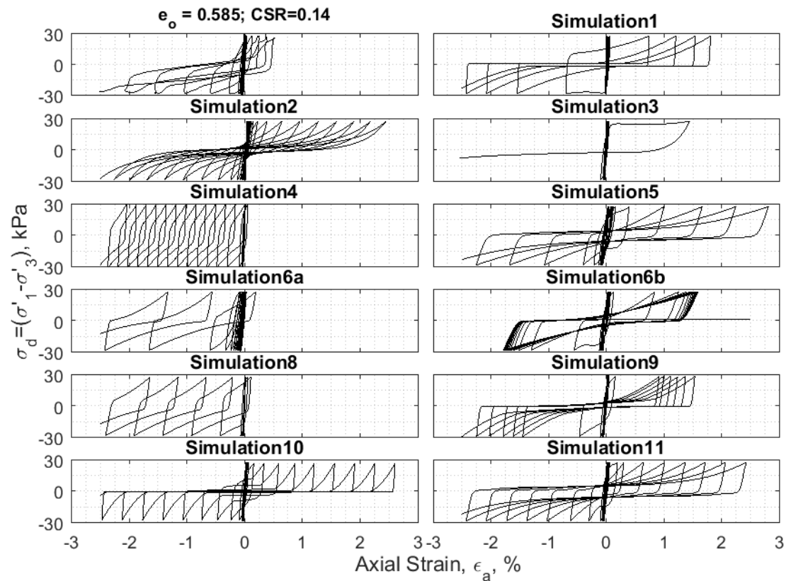
Figure 1-b. Comparison of the simulated stress-strain curves for a cyclic stress-controlled undrained cyclic triaxial test on Ottawa F65 sand. e = 0.585 ( Dr \sim 71.5\% ), p'_0 = 100 \text{ kPa} , CSR = 0.14 .
