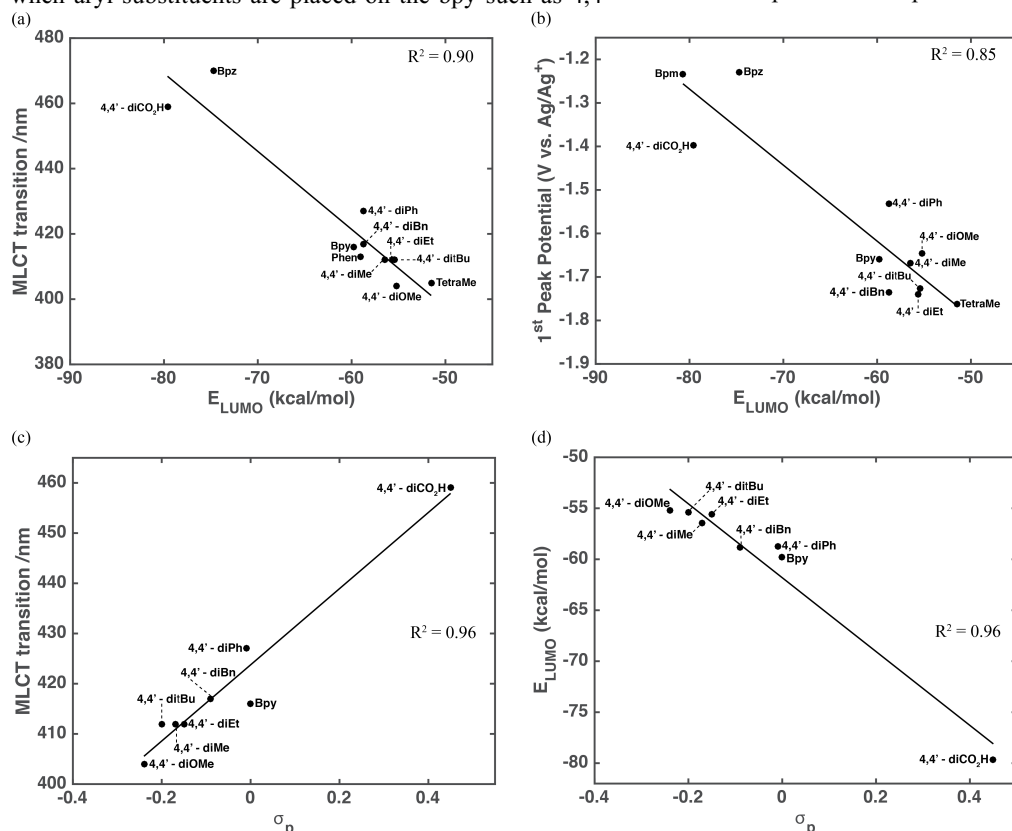
Figure 3. (a) MLCT transition wavelength vs. calculated LUMO energy. (b) First reduction peak potential vs. calculated LUMO level. (c) MLCT transition wavelength vs. para-substituted Hammett parameter ( \sigma_p ). (d) Calculated LUMO energy vs. \sigma_p .
