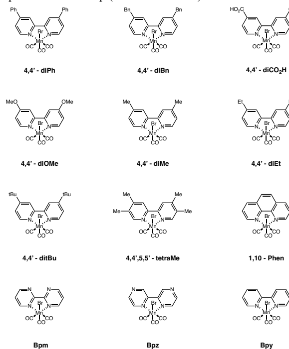
Figure 2. Scope of manganese complexes used in this study
