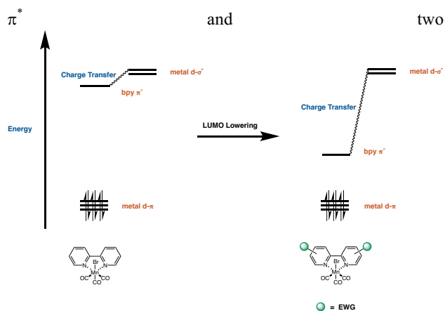
Figure 5. A schematic diagram of the effect of appending electron withdrawing groups to the bipyridine as it relates to lowering the bpy \pi^* level. EWG = electron withdrawing group.
