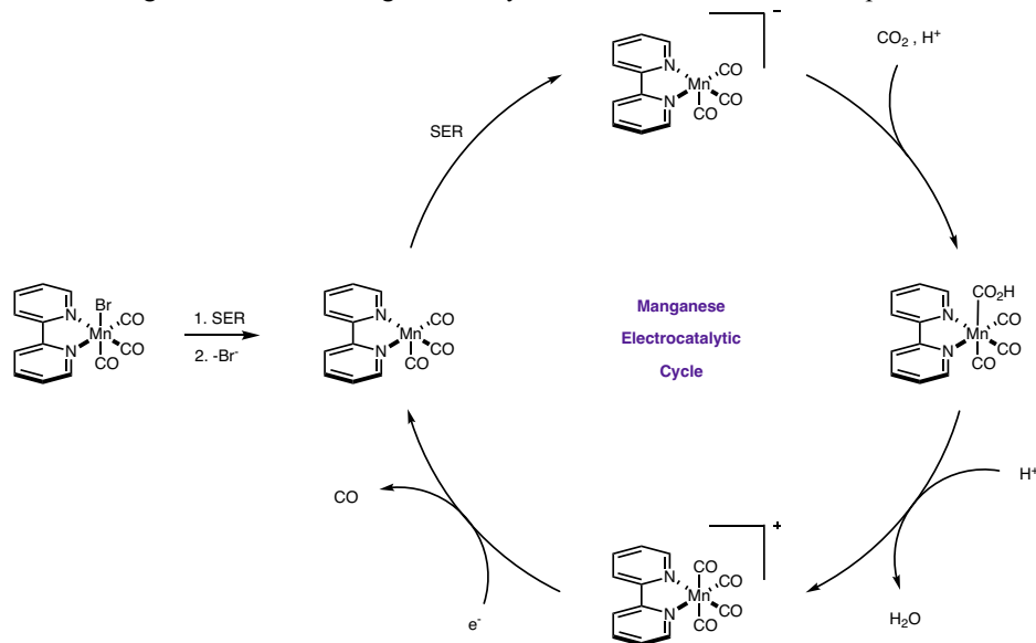
Figure 1. Catalytic Cycle for [\text{Mn}(\text{bpy})(\text{CO})_3\text{Br}] – catalyzed \text{CO}_2 reduction. SER = single electron reduction.
