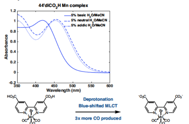
Figure 4. UV-Vis spectra of 4,4' - diCO 2 H under protonated and unprotonated conditions. Results from bulk electrolysis show that the carboxylate complex catalyzed CO 2 reduction ~3x faster than the protonated complex.
