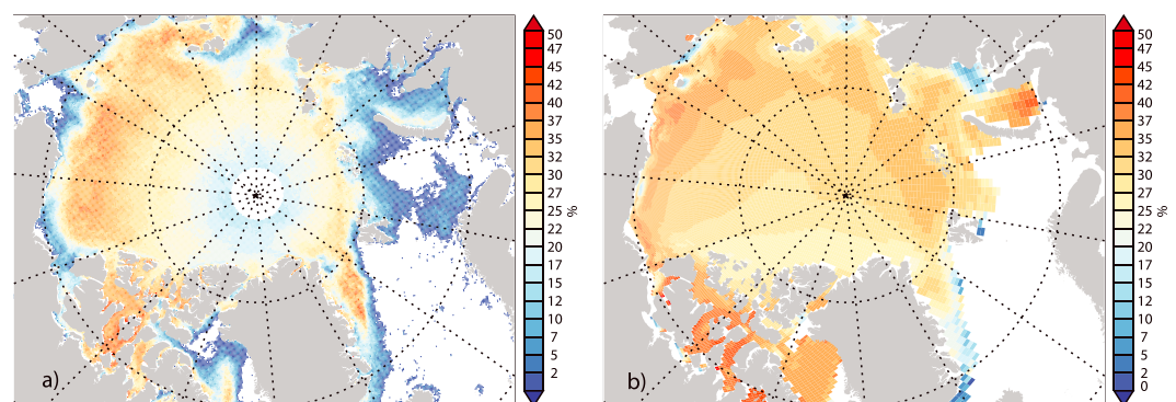
Figure 2. July 2000–2011 mean MP area fraction (%) derived from MODIS images (a) and simulated by MIZMAS (b). MODIS = Moderate Resolution Imaging Spectroradiometer; MP = melt pond; MIZMAS = Marginal Ice Zone Modeling and Assimilation System.
