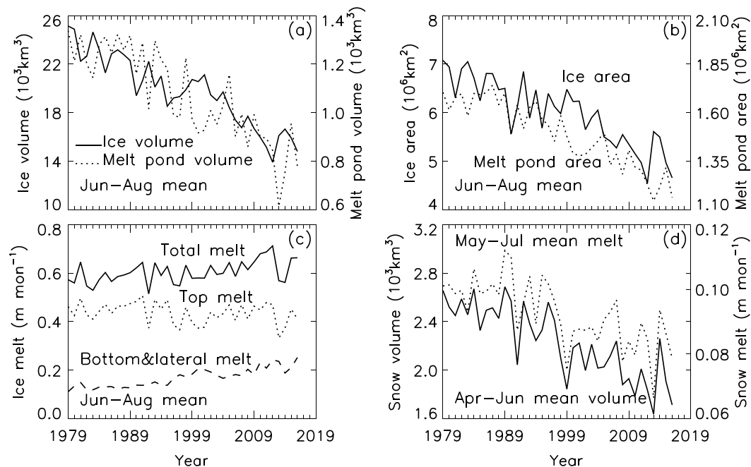
Figure 4. (a) Simulated June–August mean sea ice volume (solid line) and MP volume (dotted line), (b) sea ice area (solid line) and MP area (dotted line), (c) sea ice top melt (dotted line), bottom, lateral (dashed line), and total melt (solid line), and (d) simulated April–June mean snow volume (solid line) and May–July mean snowmelt (dotted line), averaged over the Arctic Ocean. MP volume is the integration of MP volume per unit area defined as V_p = (\rho_i/\rho_w) \int_0^\infty g_p(h)dh (see section 3) over the Arctic. Note that the snow volume and melt in Figure 4d are not averaged over the June–August period because snow has mostly melted by July (see Figure 5d). MP = melt pond.
