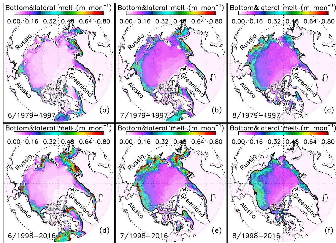
Figure 7. Simulated combined bottom and lateral melt (per unit area) for June (a, d), July (b, e), and August (c, f) averaged over the periods 1979–1997 and 1998–2016.
