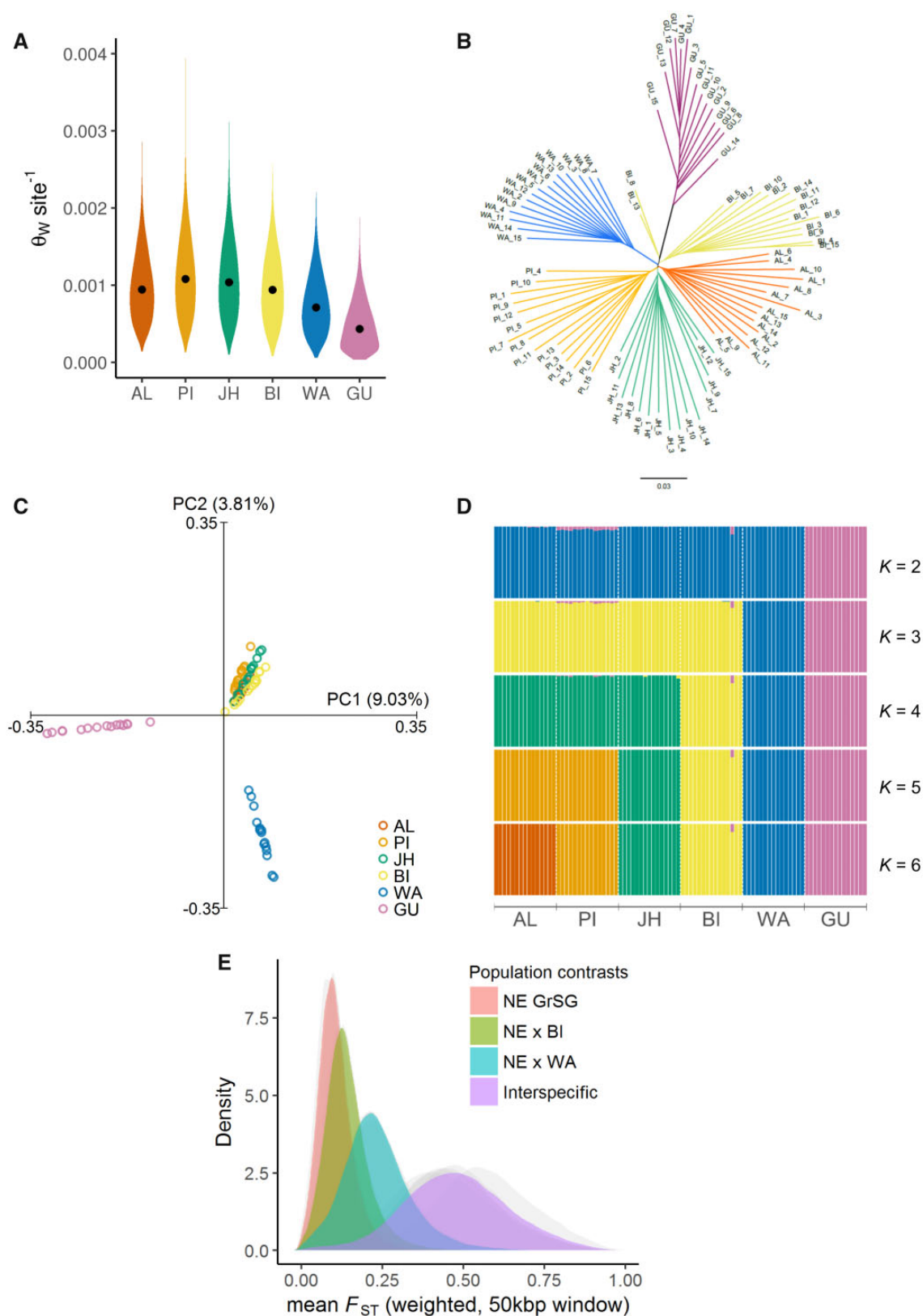
FIG. 2. —Inter- and intra-specific population genomic analyses of sage-grouse based on whole-genome resequencing. (A) Violin plots of mean per-site autosomal nucleotide diversity (Watterson's estimator, \theta_w ) across populations. Values were estimated from 50-kb sliding windows. Median values are plotted
