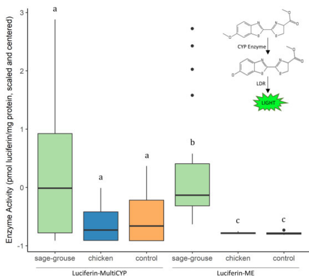
FIG. 5. —In vitro assays of sage-grouse liver enzymes. Boxplot of cytochrome P450 enzyme activity of liver microsomes from greater sage-grouse (green, n = 5 individuals), chicken (blue, n = 1 composite), and negative control (orange, n = 1 , no microsomes), from in vitro assays (four replicates per category) utilizing a nonselective cytochrome P450 substrate (Luciferin-MultiCYP) (left) and a more specific substrate (Luciferin-ME, right) that targets putative detoxification enzyme activity (CYP1 and CYP2, see Materials and Methods). Different letters above plots indicate significant differences among categories within each assay type. To aid in visual comparison, enzyme activity values have been scaled and centered within each comparison. Diagram for assay reaction (inset) wherein cytochrome P450 enzymes convert luciferin substrate (top) to luciferin methyl ester, which then produces luminescence in the presence of luciferin detecting reagent (LDR, Promega Corp.).
