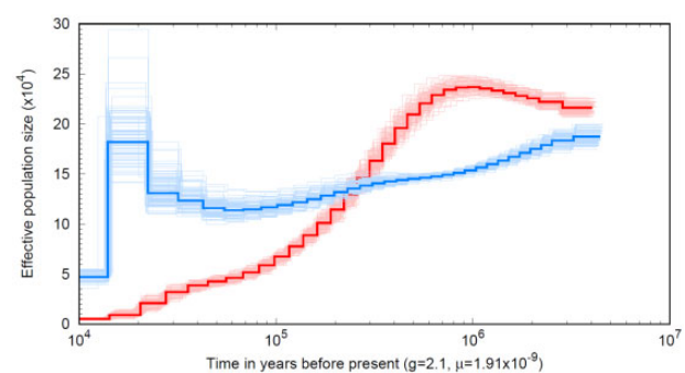
Fig. 3. —Historical changes in effective population size, from PSMC analysis of whole-genome sequences for a single Centrocerus urophasianus (blue) male and a single Centrocerus minimus (red) male. Lighter lines represent bootstrap replicates. x axis indicates (log-scale) years before present, model results were scaled based on sage-grouse generation time ( g ) and lineage-specific mutation rate ( \mu ).
