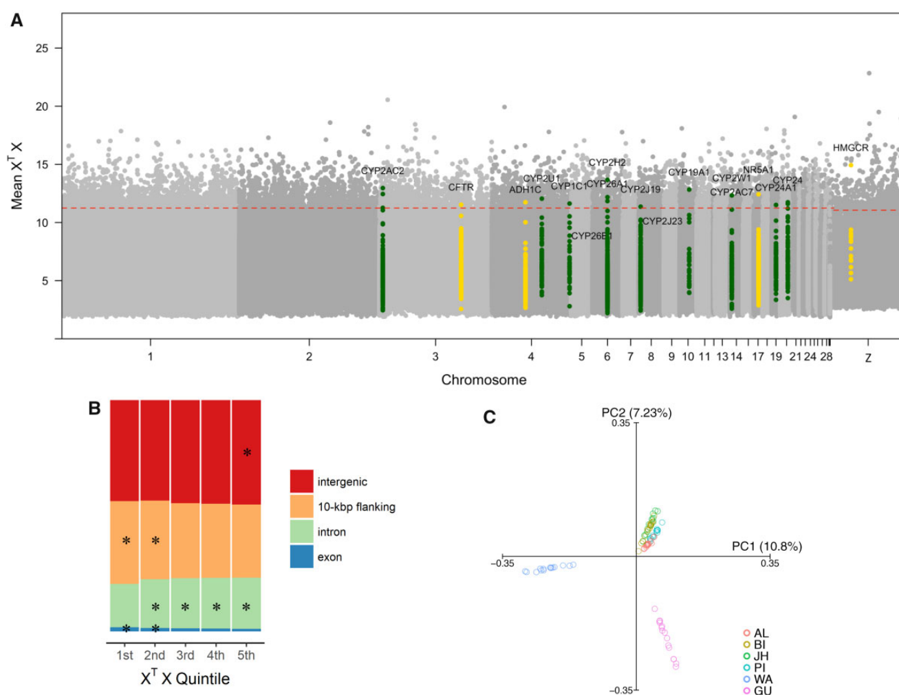
FIG. 4. —Identification and characterization of potential genomic targets of selection. (A) Manhattan plot of SNP outlier tests from whole-genome resequencing of six sage-grouse populations. Elevated X^T X values are indicative of loci with extreme population differentiation, while controlling for underlying neutral population structure. Dashed red line represents the 1% probability threshold as estimated from analysis of pseudo-observed data sets. Contrasting gray points correspond to different chromosomes based on syntenic alignment to the chicken genome. Highlighted are SNPs that occur in regions (gene \pm 10-kb flanking region) containing candidate genes for metabolic adaptation (green = cytochrome P450 genes, yellow = other important pharmacogenes). (B) Proportion of SNP effects in different genomic regions across each quintile of the observed X^T X distribution. Asterisks indicate significant overrepresentation of SNP effects in a given genomic region. (C) PCA of 1% X^T X outlier SNPs (8,592 sites). Axes represent first (PC1) and second (PC2) principal components, with percentage of total genetic variance explained by each component shown in parentheses.
