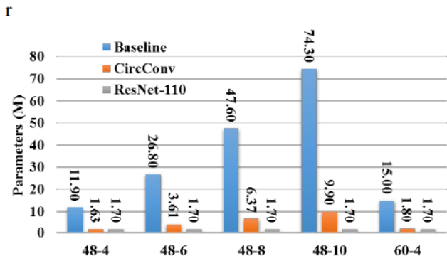
Figure 4: Wide ResNet Model Size Reduction. Compared with baseline models, compressed models achieve similar model size as ResNet-110. Compressed model named like "48-4" has 48 convolutional layers and widening parameter as 4.
