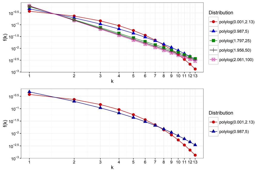
Figure 6: Polylogarithmic distributions with the same mean ( \mu = 2.67 ), but different thickness of tails. The graphs are log-log graphs, where both axes use a logarithmic scale.
