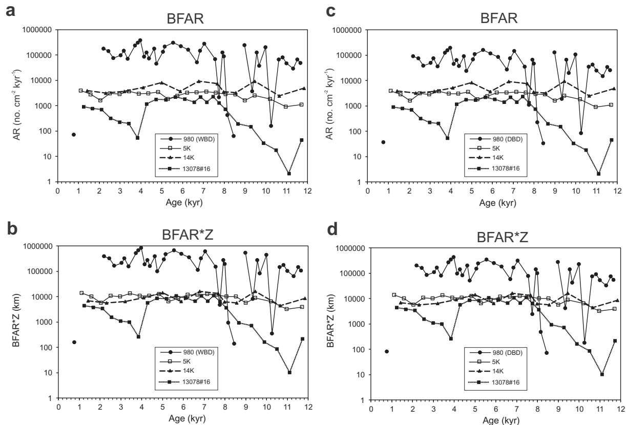
Fig. 10. (a) Comparisons of BFARs between ODP Hole 980B (calculated using wet bulk density, WBD), BOFS cores 5 K and 14 K (Thomas et al., 1995), and BENGAL core 13078#16 (Smart, 2008). Note logarithmic scale. (b) Comparisons of BFAR*Z index (calculated as BFAR multiplied by water depth, Herguera and Berger, 1991) between ODP Hole 980B (calculated using WBD), BOFS cores 5 K and 14 K (Thomas et al., 1995), and BENGAL core 13078#16 (Smart, 2008). Note logarithmic scale. (c) and (d) same as (a) and (b) respectively, apart from BFARs in ODP Hole 980B were calculated using estimated dry bulk densities (DBD).
