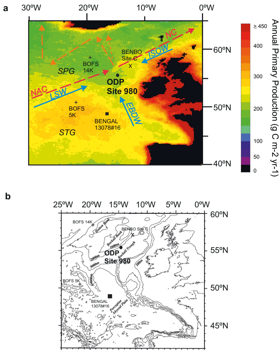
Fig. 1. Location of ODP Site 980, NE Atlantic Ocean, and of other sites mentioned in text: BENBO Site C (Gooday and Hughes, 2002), BOFS cores 5K and 14K (Thomas et al., 1995) and BENGAL core 13078#16 (Smart, 2008). (a) Surface currents are shown as dashed arrows and red text (red = warm subtropical waters, orange = cool subpolar waters); NAC = North Atlantic Current, NC = Norwegian Current, SPG = subpolar gyre, STG = subtropical gyre. Deep water currents are shown as blue solid arrows and blue text (LSW: Labrador Sea Water, ISOW: Iceland-Scotland Overflow Water, EBDW: Eastern Basin Deep Water). Satellite-derived estimates of North Atlantic mean annual productivity ( \text{g C m}^{-2} \text{yr}^{-1} ) based on SeaWiFS observations (Sun et al., 2006, Fig. 3a; Corliss et al., 2009, Fig. 1A). (b) Bathymetry of the NE Atlantic showing location of sites (modified after Lampitt et al., 2001 and Smart, 2008). (For interpretation of the references to colour in this figure legend, the reader is referred to the web version of this article.)
