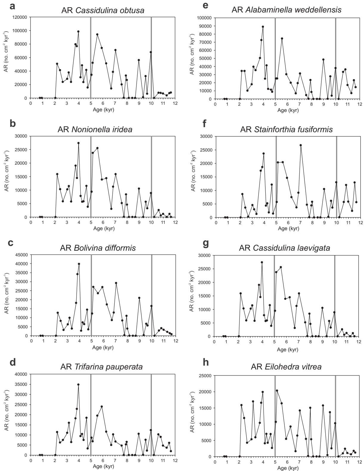
Fig. 6. Absolute abundances (AR, accumulation rates – number of specimens \text{cm}^{-2} \text{kyr}^{-1} ) of the most common species in ODP Hole 980B. ARs were calculated using WBD data (all data points included).
