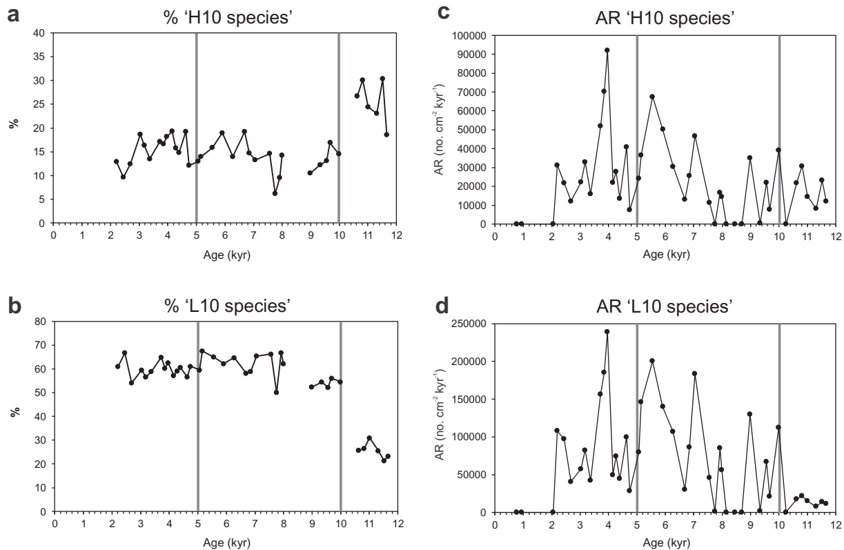
Fig. 7. (a) Relative abundances of ‘H10 species’ (i.e., species with higher % abundance before 10 ka) (combined % of A. weddellensis , S. fusiformis and T. pauperata ), and ‘L10 species’ (i.e., species with lower % abundance before 10 ka) (combined % of B. difformis , C. laevigata , C. obtusa , E. vitrea and N. iridea ). Gaps in the % records indicate samples that contained no or too few benthic foraminifera (0–13 specimens) to be used for percentage calculations. ARs were calculated using WBD data (all data points included).
