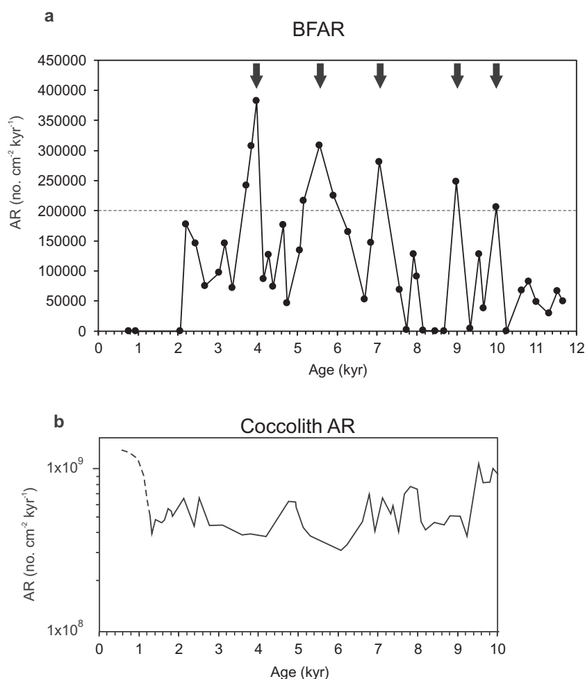
Fig. 9. Comparison between (a) BFARs (calculated using WBD data), and (b) coccolith accumulation rates (AR, calculated using WBD data) (modified after Berger et al., 2014, Fig. 10c) in ODP Site 980. Arrows in (a) show peaks in BFARs ( > 200,000 \text{ cm}^{-2} \text{ kyr}^{-1} ).
