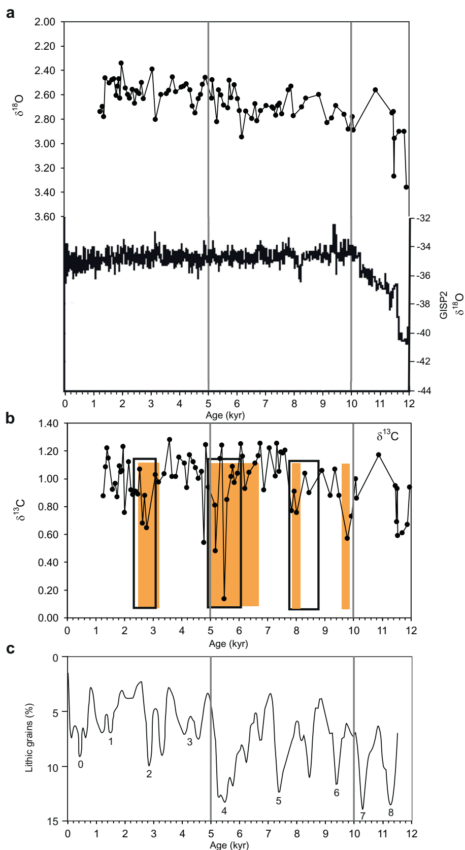
Fig. 2. (a) Benthic \delta^{18}\text{O} records for ODP Hole 980B (left axis) (Oppo et al., 2003, 2007) compared with oxygen isotope data from the Greenland Ice Sheet Project 2 (GISP2) ice core (right axis) (Dansgaard et al., 1993; deMenocal, 2001, fig. 2A), (b) benthic \delta^{13}\text{C} records for ODP Hole 980B (Oppo et al., 2003, 2007), (c) Percentage of lithic grains (ice-rafted debris, 63–150 \mu\text{m} size range) from stack of cores MC52-V29191 + MC21-GGC22 (4 records) showing North Atlantic Bond events (numbered) (Bond et al., 2001, fig. 2). Shading in (b) shows low \delta^{13}\text{C} events and possible correlative events in the other records; rectangles, denote extreme winter-like conditions from GISP2 (Oppo et al., 2003, fig 1; O'Brien et al., 1995).
