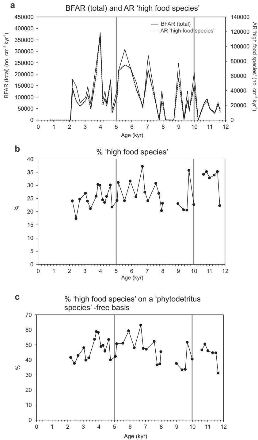
Fig. 8. (a) Comparison between BFARs (total) and accumulation rates of 'high food species' (sum of Abditodentrix spp., Bolivina spp., Bolivinelina spp., Brizalina spp., Bulimina spp., Globobulimina spp., Melonis spp., Stainforthia spp., T. pauperata and Uvigerina spp.), (b) relative abundances (%) of 'high food species', and (c) % of 'high food species' calculated on a 'phytodetritus species'-free basis in ODP Hole 980B. ARs were calculated using WBD data (all data points included). Gaps in the % records indicate samples that contained no or too few benthic foraminifera (0–13 specimens) to be used for percentage calculations.
