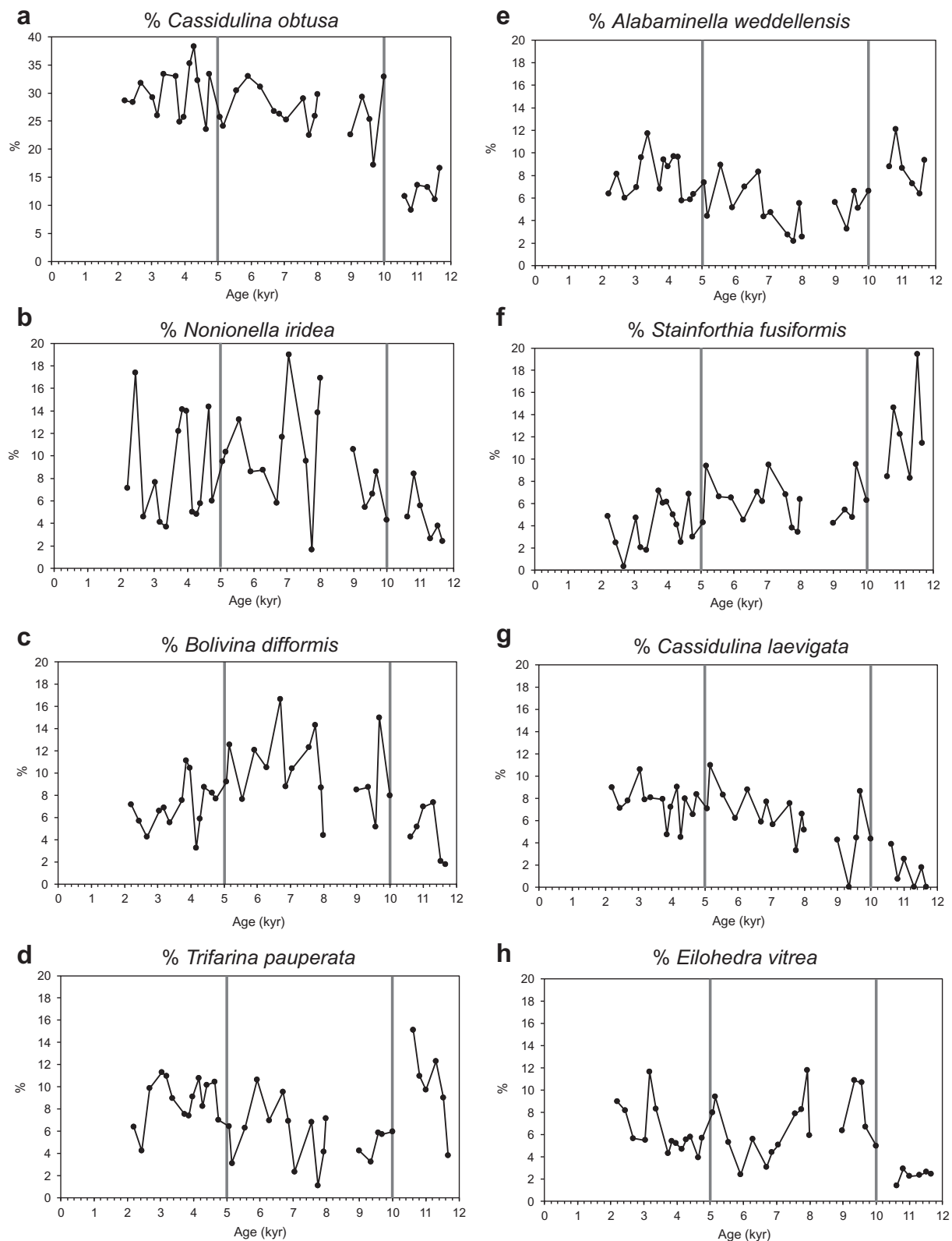
Fig. 5. Relative abundances (%) of the most common species in ODP Hole 980B. Gaps in the % records indicate samples that contained no or too few benthic foraminifera (0–13 specimens) to be used for percentage calculations.
