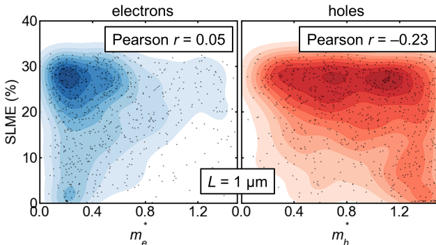
Figure 6: Scatter plots of SLME at L = 1 \mu\text{m} absorber thickness against electron and hole effective masses for \approx 800 phases passing the intermediate screens. From the Pearson correlation coefficients (annotated) the electron mass is seen to be essentially uncorrelated with SLME, while the hole mass has a fortuitous, moderately negative correlation with SLME: A higher SLME is associated with lighter holes. This is primarily driven by the underlying correlations between carrier masses and band gap (see Figure S4). Blue and red shading indicate the 2-D distribution of the points (via kernel density estimation).
