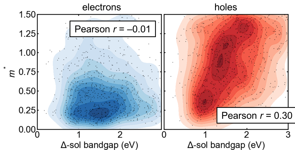
Figure S4: Scatter plots of effective mass versus bandgap for the \approx 800 phases passing the intermediate screens. Pearson correlation coefficients reveal that electron mass is essentially uncorrelated with bandgap, while there is a modest tendency for narrower gap materials to exhibit lighter holes. A discussion of likely chemical origins of this behavior and its consequences for SLME is given in the main text. Blue and red shading indicate the 2-D distribution of the points (via kernel density estimation).
