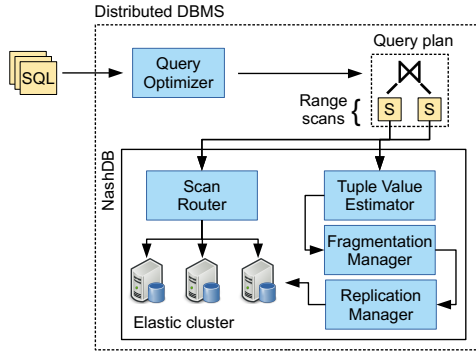
Figure 1: NashDB system architecture
