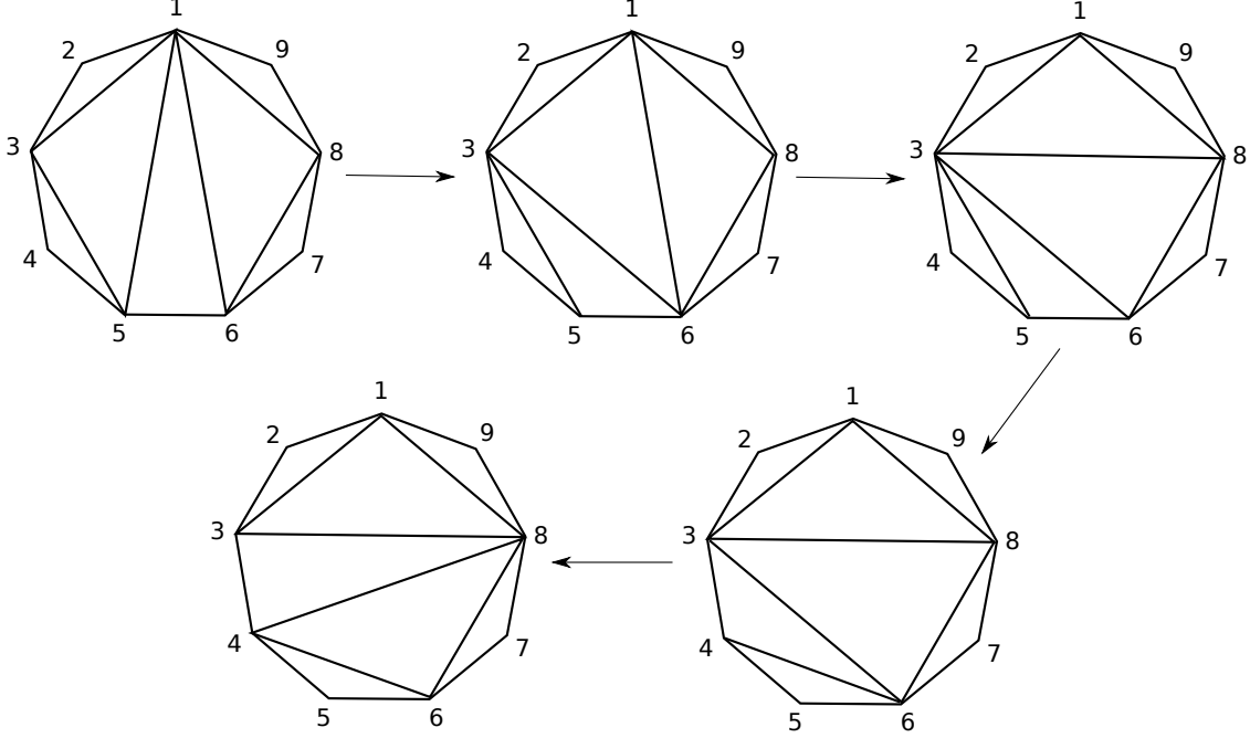
Figure 12: Monodromy action via a sequence of flips of triangulations of the 9-gon.
