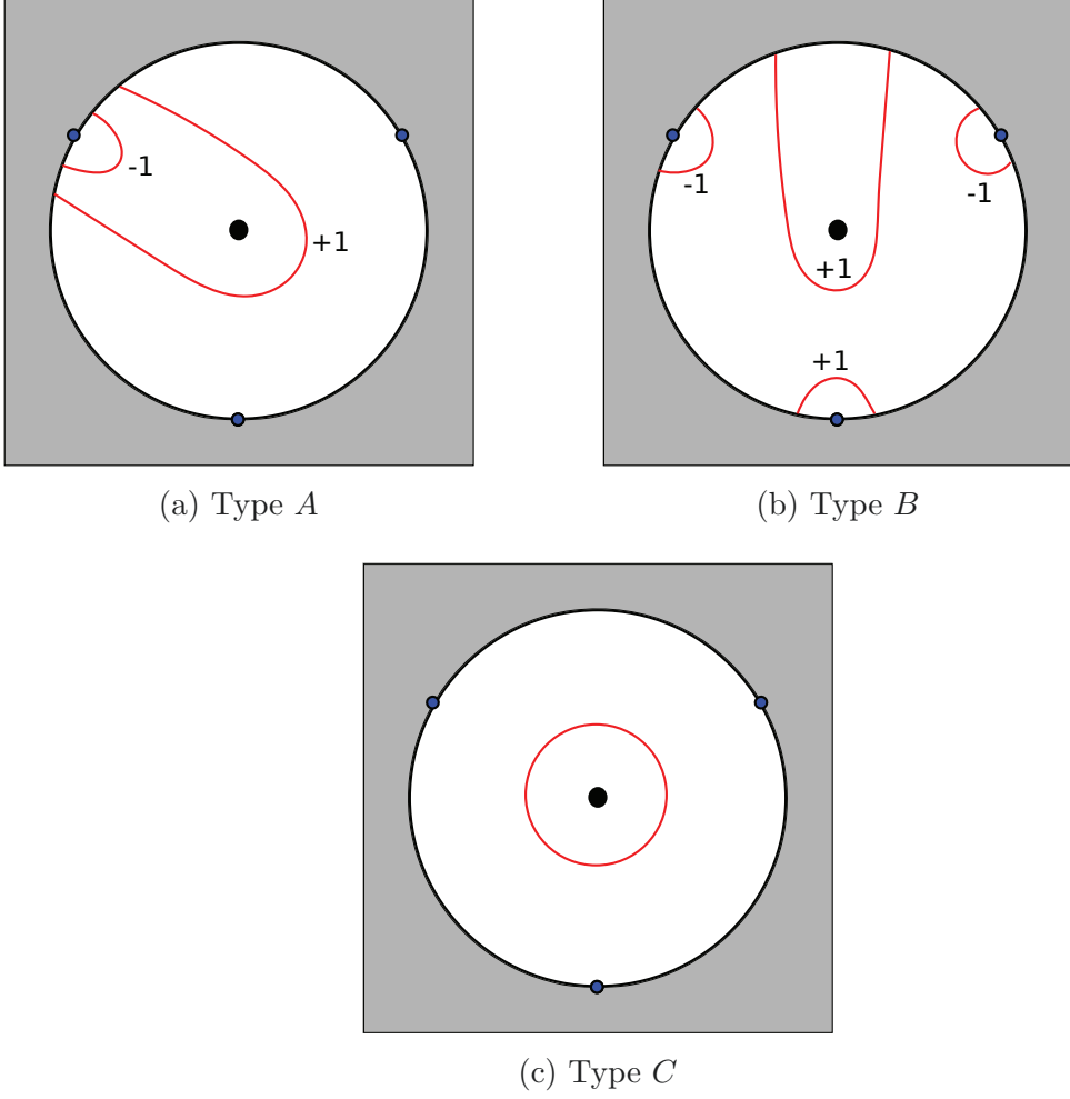
Figure 15: Three types of laminations in (A_1, D_3) Argyres-Douglas theory.
