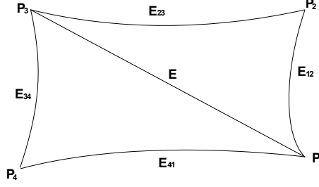
Figure 1: The quadrilateral Q_E associated to edge E .
