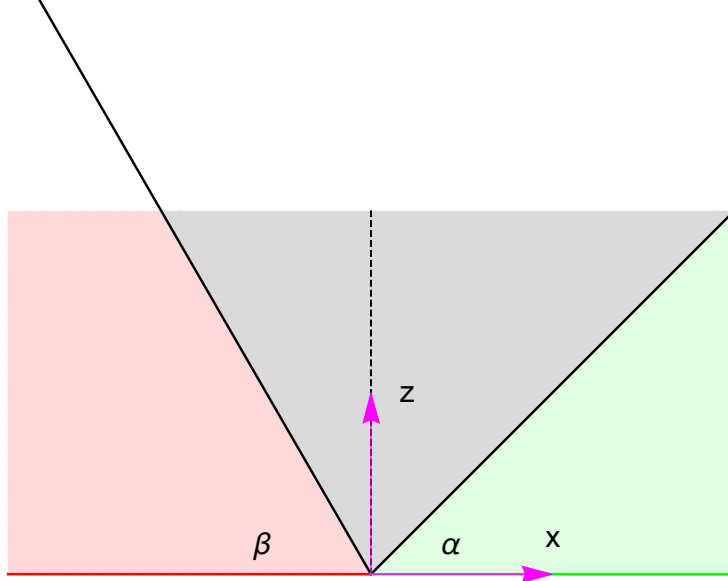
Figure 3. A thin wall geometry consists of two wedges of pure \text{AdS}_3 (pink and green regions) glued along a tensionful wall. The wall occupies a ‘straight line’ in the Poincaré coordinates, which delimits each \text{AdS}_3 chunk. The two straight lines are identified.
