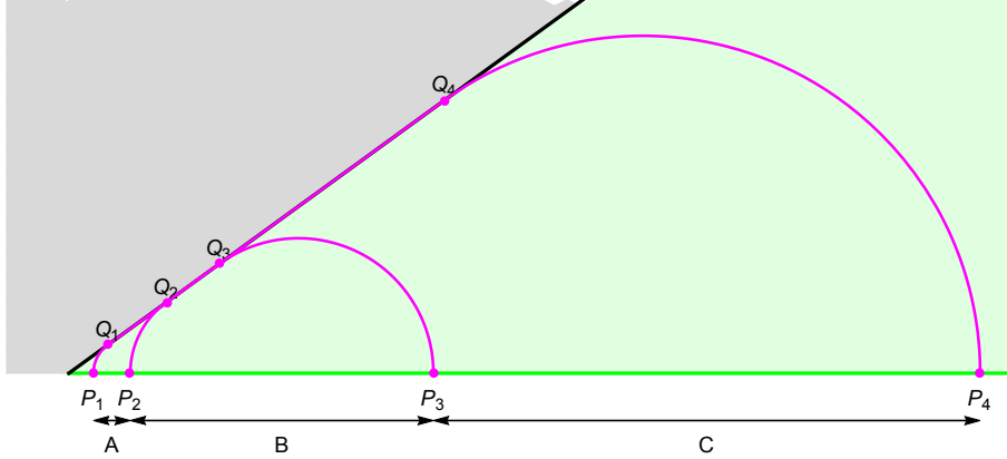
Figure 4. A wall-crossing geodesic in a thin wall geometry consists of two arcs, which meet the wall at the same angle and location.
