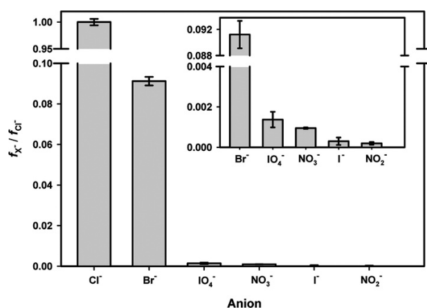
Figure 5. Anion fractionation factor, f_X^- , normalized relative to the fractionation of chloride, f_{Cl^-} , for molar ratios of anions found in seawater. A comparison to bulk seawater value indicates that at the air–water interface, iodide and bromide can be respectively enriched by 7.3 \times 10^3 and 7.5 \times 10^2 times. Reproduced with permission from reference [134].
