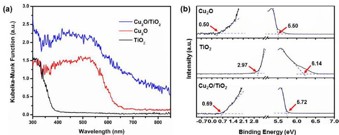
Fig. 4. (a) UV-visible absorption spectra for solid samples. (b) UPS spectra for \text{Cu}_2\text{O} octahedral (top), pure \text{TiO}_2 (center), and \text{Cu}_2\text{O}/\text{TiO}_2 heterostructure (bottom). Extrapolations to the left and right hand sides correspond to the onset values for the valence band and secondary electron spectra, respectively. A complete description is available in the Supporting Information (see Fig. S5).
