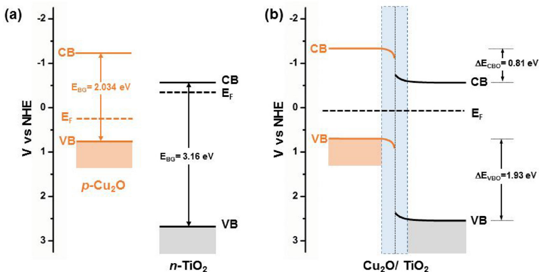
Fig. 5. Energy band diagrams for (a) \text{Cu}_2\text{O} and \text{TiO}_2 before contact and (b) \text{Cu}_2\text{O}/\text{TiO}_2 composite.
