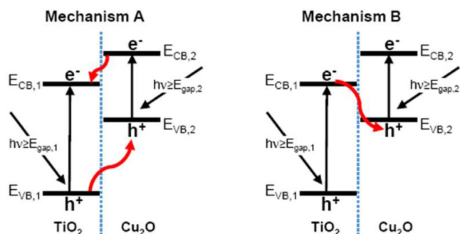
Scheme 1. Schematic representation of the processes that can take place in a system consisting of two semiconductors in electrical contact under irradiation with photons of suitable energy. (A) Double-charge transfer, and (B) direct Z-scheme mechanism.
