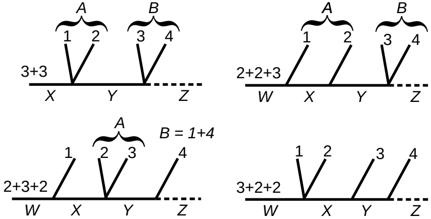
Figure 1. All 5-body decays with one or more 3-body vertices. The labels A and B are used throughout the text to refer to groupings of particles when convenient.
