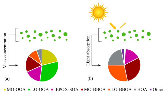
Figure 15. Comparative relationship of the relative contributions of PMF factor loadings to (a) organic PM 1 mass concentration and (b) organic PM 1 light absorption. Results represent means for the full data sets of IOP2. The means and standard deviations are listed in Table 4. Results are for 370 nm. “Other” refers to the model intercept B (Eq. 5).
