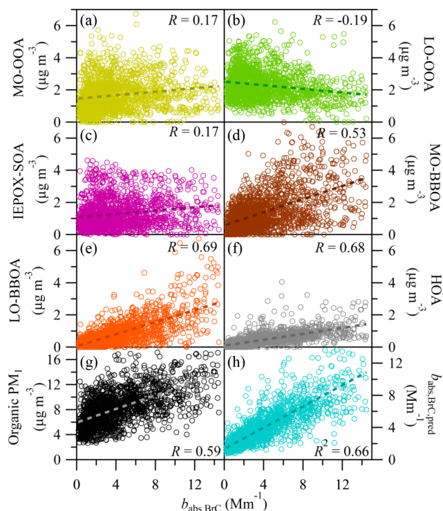
Figure 14. Scatter plots against b_{\text{abs,BrC}} of (a)–(f) PMF factor loadings, (g) organic \text{PM}_1 mass concentration, and (h) b_{\text{abs,BrC,pred}} values predicted by a multivariate linear regression model using PMF factor loadings as parameters as described by Eq. (5).
