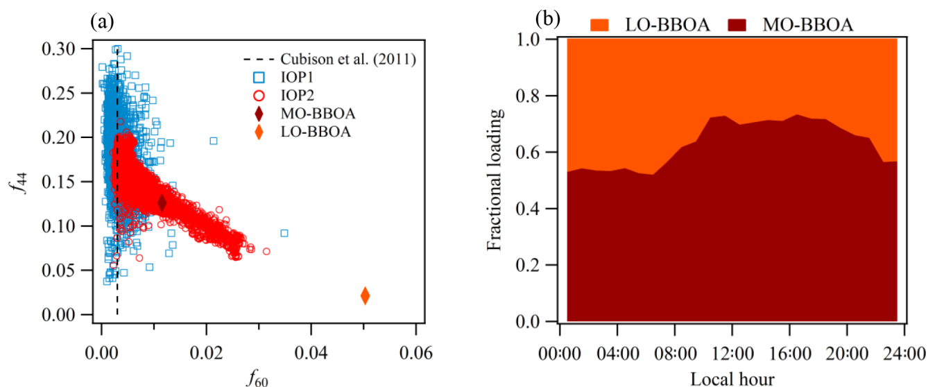
Figure 7. Analysis of the organic PM_1 sampled at the T3 site in relation to biomass burning. (a) Scatter plot of the AMS signal fraction at m/z 44 ( f_{44} ) against that at m/z 60 ( f_{60} ). Red circles represent measurements during the dry season (IOP2), and blue squares represent measurements at the same site during the wet season (IOP1) (de Sá et al., 2018). Diamonds represent the MO-BBOA and LO-BBOA factors of IOP2. The dashed line represents a reference for negligible influence by biomass burning based on several field studies (Cubison et al., 2011). (b) Diel trends of the fractional loadings of the MO-BBOA and LO-BBOA factors relative to their sum BBOA_T . Local time is UTC minus 4 h.
