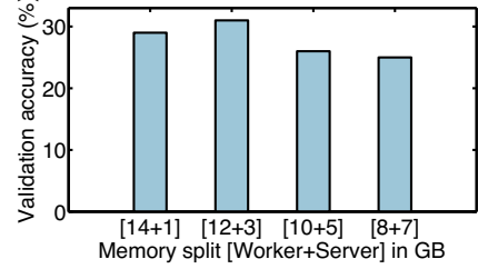
Figure 4: Effect of memory allocation with co-location
