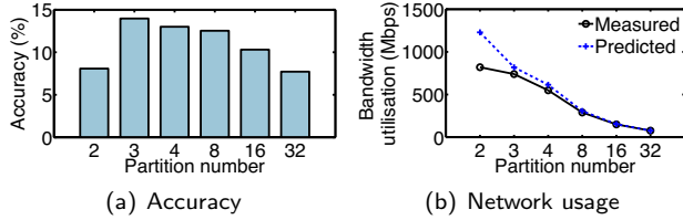
Figure 12: Effect of gradient partitions
