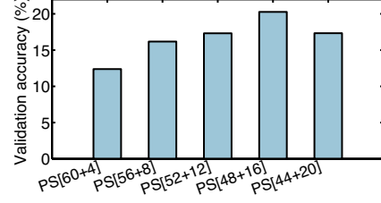
Figure 2: Accuracy for different worker/parameter server allocations in cluster
