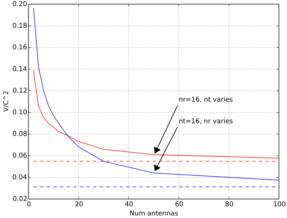
Fig. 3. Normalized dispersion \frac{V}{C^2} as a function of n_r and n_t . The received power is P_r = 20\text{dB} and T = 16 . Dashed lines are asymptotic values from (266)-(269).
