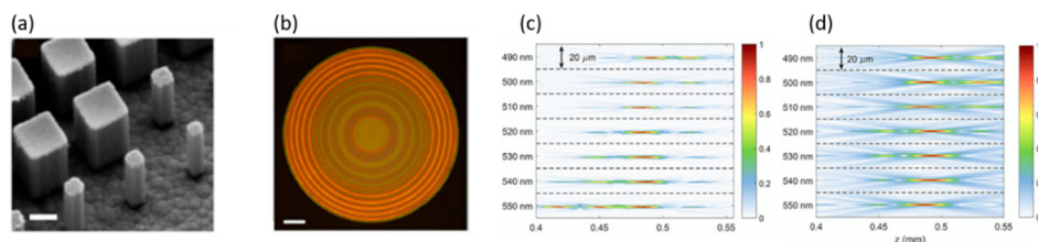
Figure 5. A 60 nm bandwidth achromatic metalens. (a) Side view scanning electron microscope (SEM) image of the fabricated AML, scale bar: 200 nm. (b) Optical image of the AML. Scale bar: 25 \mu\text{m} . (c) Measured intensity profiles of the reflected beam by the AML in the xz -plane at different wavelengths. (d) Simulated intensity profiles of the reflected beam by the AML in the xz -plane at different wavelengths. (Reproduced from [32] with permission.)
