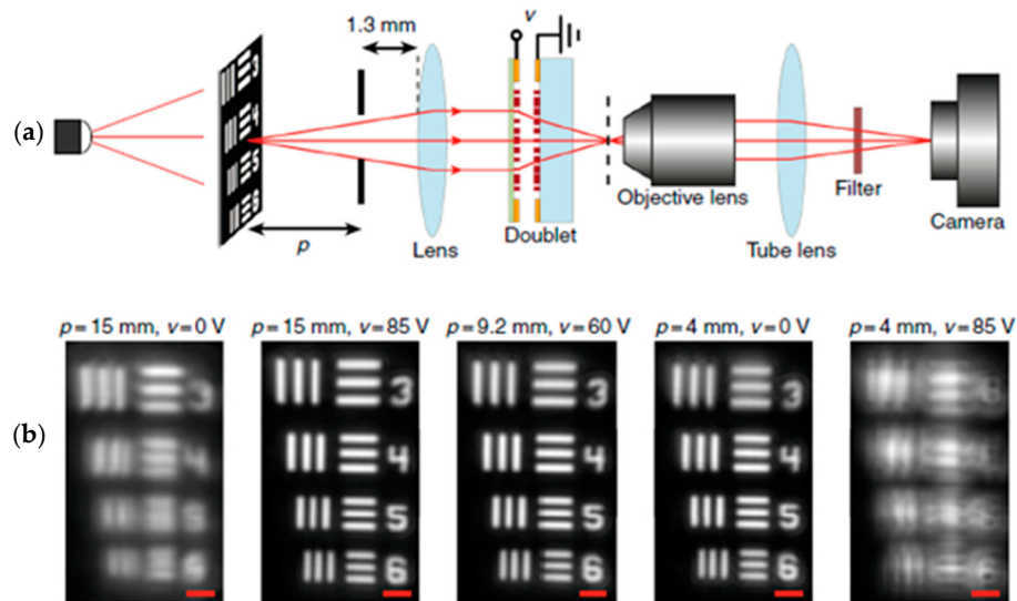
Figure 10. Imaging with the tunable doublet. (a) Schematic illustration of the imaging setup using a regular glass lens and the tunable doublet. The image formed by the doublet is magnified and re-imaged using a custom-built microscope with a \times 55 magnification onto an image sensor. (b) Imaging results, showing the tuning of the imaging distance of the doublet and glass lens combination with applied voltage. By applying 85 V across the device, the imaging distance increases from 4 to 15 mm. The scale bars are 10 \mu\text{m} . (Reproduced from [49] with permission.)
