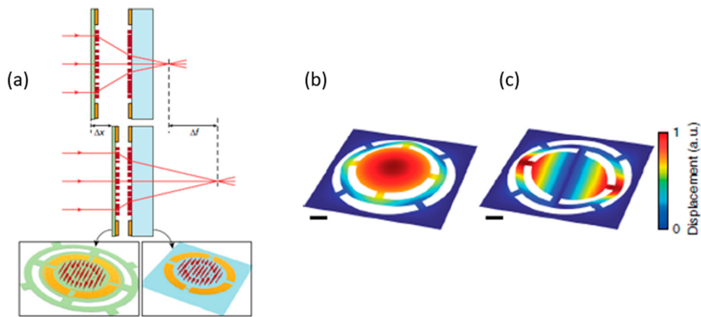
Figure 9. Metasurface-based MEMS device with tunable focus. (a) Schematic illustration of the proposed tunable lens, comprised of a stationary lens on a substrate, and a moving lens on a membrane. The first (b) and second (c) mechanical resonances of the membrane at frequencies of 2.6 and 5.6 kHz, respectively. The scale bars are 100 \mu\text{m} . (Reproduced from [49] with permission.)
