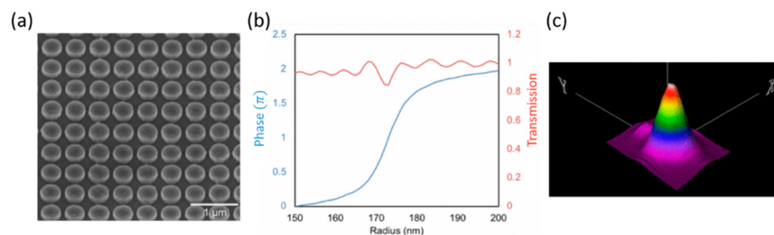
Figure 14. Metalens-based confocal microscope system. (a) \text{TiO}_2 nanoresonator array. (b) Phase and transmission vs. nanodisc radius by FDTD simulation. (c) a 3D intensity laser-focused spot profile. (Reproduced from [93] with permission.)
