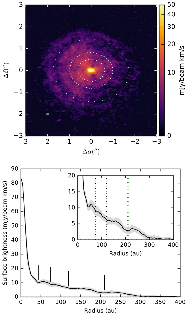
Figure 5. Moment-zero map (top panel) and azimuthally averaged deprojected radial profile (bottom panel) of the ^{12}\text{CO } 2 - 1 line emission. Emission with S/N lower than 3 has been clipped. Only the uncontaminated east part of the image was considered to create the deprojected profile. The four vertical bars mark the position of the CO gaps. The two white (black in the lower panel) dotted lines mark the position of the prominent outer dust rings, located at 75 and 120 au, and the green dotted line marks the position of the outermost CO gap near 210 au.
