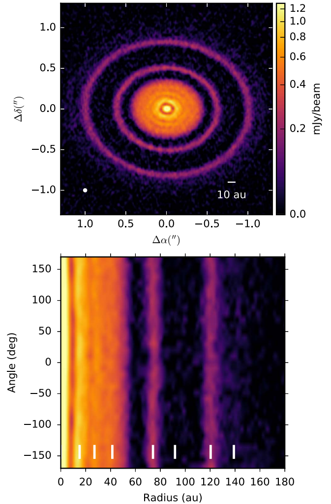
Figure 1. Dust continuum emission map (upper panel), and the deprojected emission shown in polar coordinates (bottom panel), using an inclination of 34^\circ 88' and a position angle of 85^\circ 76' . The beam of 0''.03 \times 0''.04 is shown in the bottom left, corresponding to a spatial resolution of 3.6 \times 4.8 au. The white vertical bars in the bottom panel locate the position of the rings.
