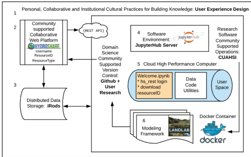
Fig. 1. Illustration of six basic elements for a knowledge infrastructure for interactive community modeling and exploration. Research software communities maintain support of operations between Docker Containers and software environment. Domain science communities maintain support for version control and user communications specific to modeling frameworks.
