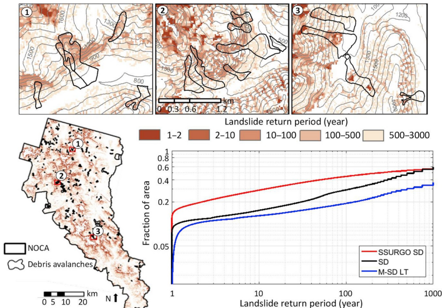
Fig. 4. Maps show modeled landslide return periods using Landlab for NOCA overlain with mapped debris avalanches, including zoomed in areas at top for greater detail. The uncertainty of soil depth was characterized from a long-term soil evolution model (M-SD LT). Cumulative distribution of landslide return periods for SSURGO soil depth (SSURGO-SD), modeled soil depth (M-SD), and modeled soil depth considering long-term dynamics (M-SD LT) scenarios, plotted on a log-log scale using the Weibull plotting position. (Figure adapted in entirety from Strauch et al., 2018 under CC BY 4.0).
