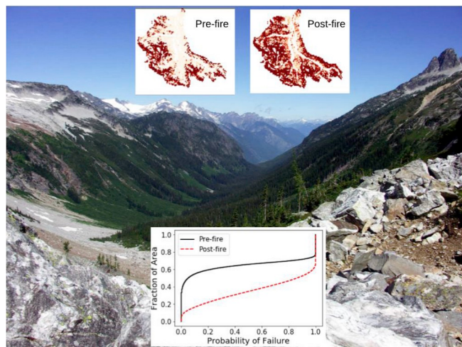
Fig. 5. Landslide probability estimates in the Thunder Creek watershed (photo) increase given post-fire root cohesion assumptions (70% less), as compared to the original cohesion assumptions in Strauch et al. (2018) . As an example of knowledge infrastructure functionality, the notebook replicates published findings, as well as tests the parameter function described in the peer-reviewed publication. Inset maps and cumulative distribution plots of the spatial probability of landsliding for pre-fire and post-fire conditions. Photo is looking north down the broad, glacial carved valley of Thunder Creek (courtesy of Michael Kirshenbaum and National Park Service).
