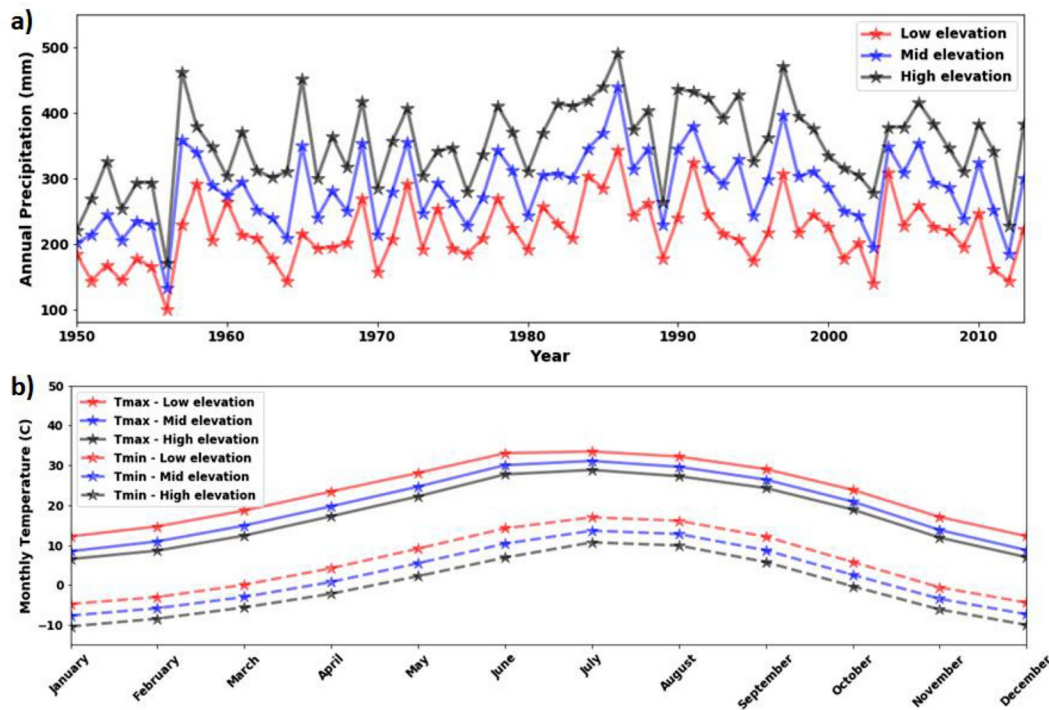
Fig. 7. Climate data downloaded and processed from Livneh et al. (2015). a) Annual precipitation plotted with respect to time for each elevation band. b) Mean monthly daily minimum and maximum temperatures for each elevation band.
