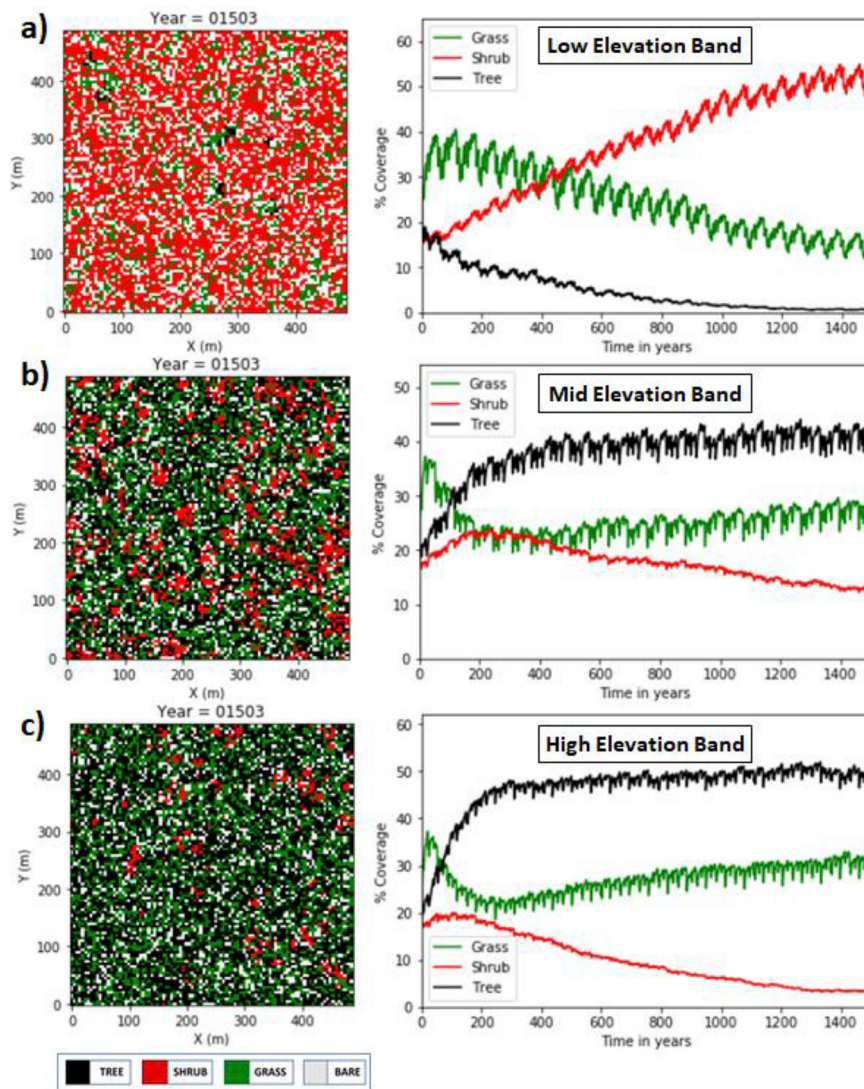
Fig. 8. Spatial Organization of PFTs at year 1503 (left column) and Annual areal cover fraction of each PFT plotted with respect to time (right column) for; a) low elevation landscapes (1200 m–1700 m), b) mid elevation landscapes (1700 m–2000 m), and c) high elevation landscapes (2000 m–2500 m).
