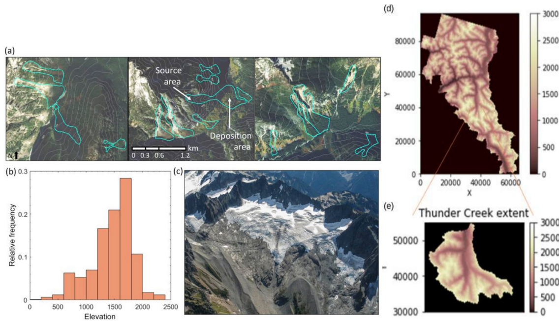
Fig. 3. (a) Example debris avalanches (cyan) mapped in three areas within NOCA. Contours are in 100 m intervals. Aerial image source from World Imagery, Esri Inc.; (b) elevation distribution of the relative frequency of mapped debris avalanche source areas; and (c) High elevation rock and glacier surrounding Spiral Glacier in North Cascades showing a bedrock glacier cirque with thin barren soils and moraine deposits (photo by John Scurlock with permission), (d) elevation (ft) for NOCA model extent from Strauch et al. (2018) , and (e) for the subset for the Thunder Creek extent. (Figures a–c adapted in entirety from Strauch et al., 2018 under CC BY 4.0). (For interpretation of the references to colour in this figure legend, the reader is referred to the Web version of this article.)
