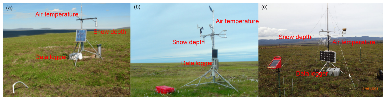
Figure 2. Typical permafrost observing stations. (a) Imnaviat site (68.64° N, 149.35° W) in the GI-UAF network (source: http://permafrost.gi.alaska.edu/site/im1 , last access: 15 December 2018); (b) the Drew Point station (70.86° N, 153.91° W) in the USGS network (source: http://pubs.usgs.gov/ds/0977/DrewPoint/DrewPoint.html , last access: 15 December 2018); (c) the Wigand site (63.81° N, 150.109° W) in the NPS network.
