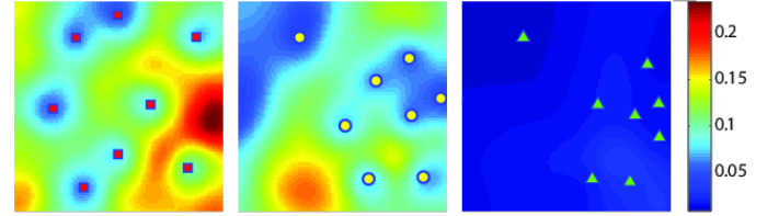
Fig. 8: The error of estimated spectrum in the area of interest corresponding to Fig. 7. (Left) RIP based, Algorithm 1. (Middle) Online RIP based, Algorithm 2 while only 5% of sensors are sensed. (Right) Centralized RIP based, Algorithm 2 while all the sensors are sensed. \lambda is assumed 0.7
