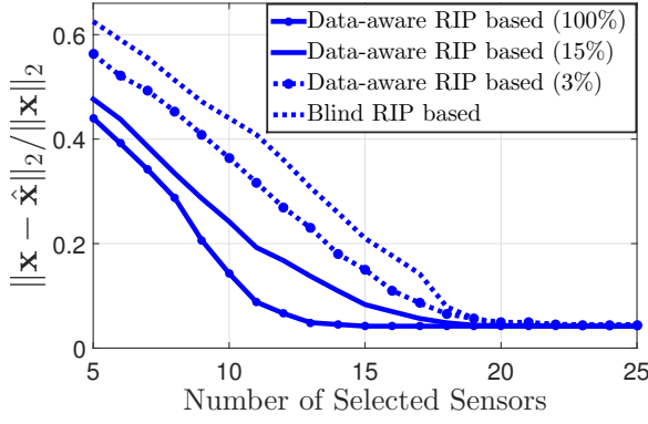
Fig. 5: Performance of blind and data-aware RIP based sensor selection algorithms in terms of number of selected sensors.
