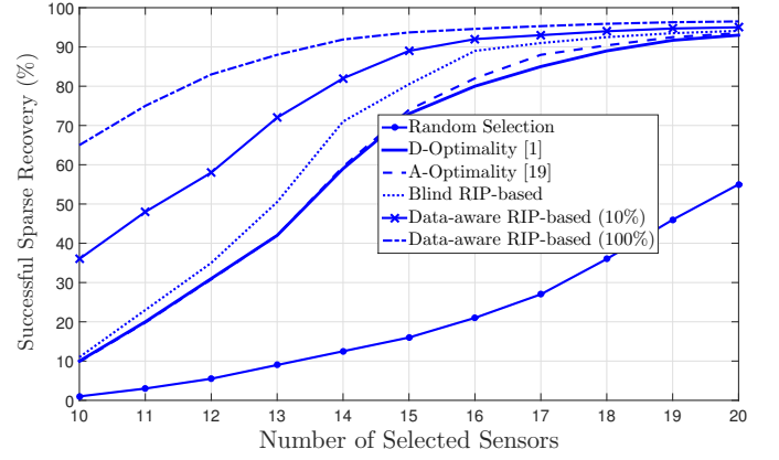
Fig. 3: Performance of different sensor selection algorithms in terms of number of selected sensors
