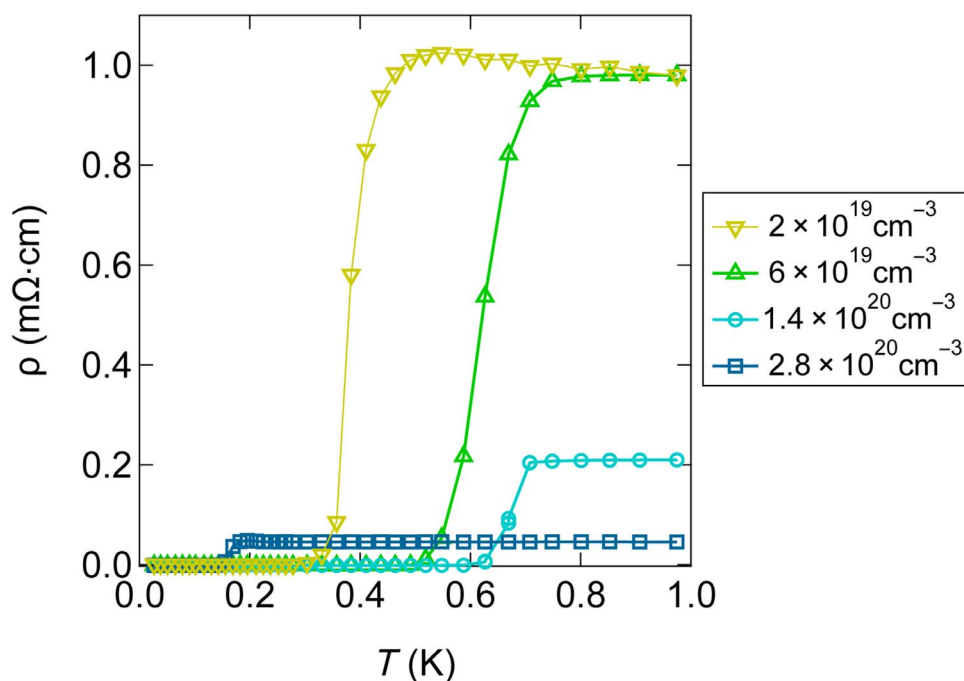
Fig. 2. Superconducting transitions for strained Sm-doped \text{SrTiO}_3 films with different carrier densities. The resistivity as a function of temperature between 1 K and 10 mK without an applied magnetic field is shown. The legend indicates the Hall carrier densities measured at 300 K. Lines are a guide for the eye.
