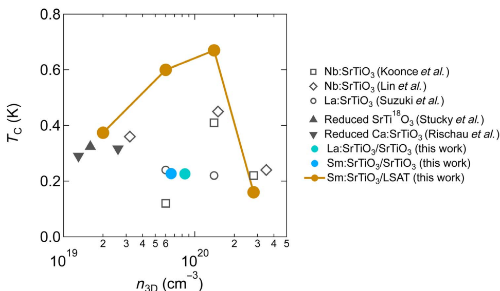
Fig. 3. Comparison of T_C of strained and unstrained \text{SrTiO}_3 . T_C values of strained and unstrained La- and Sm-doped \text{SrTiO}_3 films with different carrier densities grown on LSAT and \text{SrTiO}_3 substrates, respectively (filled circles), are shown. T_C values of \text{SrTiO}_3 crystals taken from the literature are also shown, some of which were tuned toward a ferroelectric transition (triangles). Literature data are from Lin et al. (11), Stucky et al. (25), Rischau et al. (26), Koonce et al. (33), and Suzuki et al. (34). Lines are a guide for the eye.
