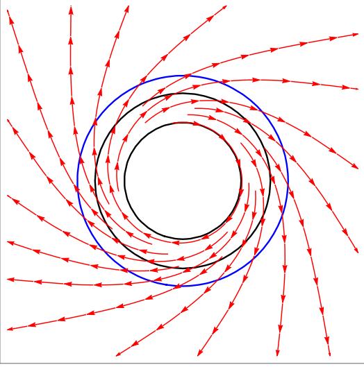
FIG. 2. Electric field lines for the field 13, with r_+ = 0.3 , r_- = 0.2 , and \Omega_F = \Omega_H/2 = 1/3 , in units with \ell = 1 . As explained in Appendix C, the field lines are intersections of the electric field sheets with a surface of constant ingoing Kerr coordinate v , plotted with r and \phi treated as polar coordinates on the Euclidean plane. The field lines for r < r_- are not plotted, since F_3 is singular at r_- .
