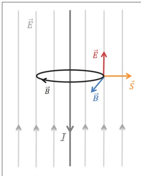
FIG. 1. A line current driven opposite to an ambient electric field emits a Poynting flux of energy. This field configuration corresponds to (2). Its generalization to a any stationary axisymmetric spacetime (1), allowing for a radial component of the magnetic field, is given by (4). For spinning black cylinder spacetimes, the line current is behind the horizon, and the field is nonsingular on the horizon provided the Znajek condition (9) holds. Energy is then extracted from the black cylinder if there is magnetic flux through the horizon and 0 < \Omega_F < \Omega_H (10). The nonzero black hole spin is what makes this extraction possible.
