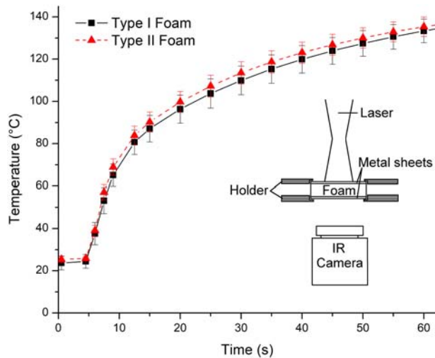
Fig. 9 Foam pucks were sandwiched between two solid aluminum disks. A laser with spot size D = 12 mm was applied to the top surface of the assembly and the temperature was measured underneath. The measured heat diffusion through the type I and type II foams was very similar. The results were averaged over two specimens that were tested from both directions, standard deviations are shown.
