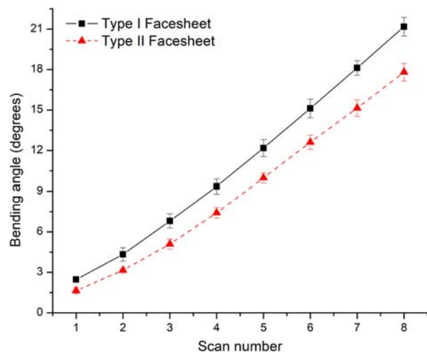
Fig. 7 Bending angles of the “isolated” facesheets (not attached to foam core) at a small spot size ( D = 4 mm, v = 30 mm/s). The type I facesheet, made of AW 5005, bent more efficiently than the type II facesheet, which was made of Al 1060.
