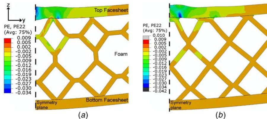
Fig. 15 Plastic strain distributions in the y -direction in a Kelvin-cell sandwich model after a laser scan at a large spot size ( D = 12 mm, v = 10 mm/s). Only half of the model is shown due to symmetry. In (a), the foam core was constructed such that cavities are underneath the top facesheet at the symmetry plane, whereas in (b), mostly cell walls are underneath the top facesheet. The remaining properties of both models are identical. The deformation was scaled by a factor of 10 for viewing clarity.
