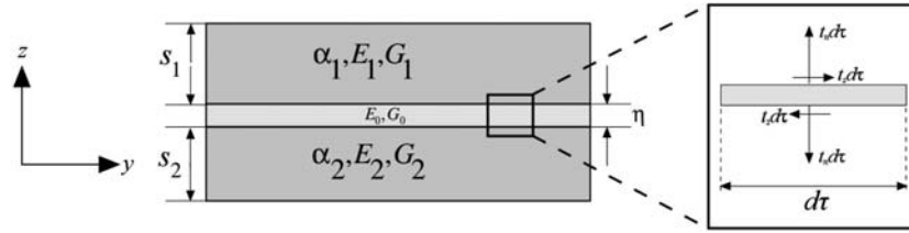
Fig. 2 Schematic of two layers of thicknesses s_1 and s_2 that are joined by an interface of thickness \eta , with a close-up of the traction components at the interface [13]
