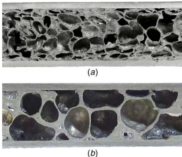
Fig. 1 (a) Type I sandwich panel and (b) type II sandwich panel
