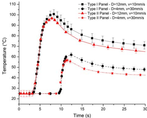
Fig. 11 Temperature history on the bottom surface of the sandwich panels during laser scans at a large spot size ( D = 12 mm, v = 10 mm/s) and a small spot size ( D = 4 mm, v = 30 mm/s). Four specimens were tested for each sandwich panel type, standard deviations are shown.
