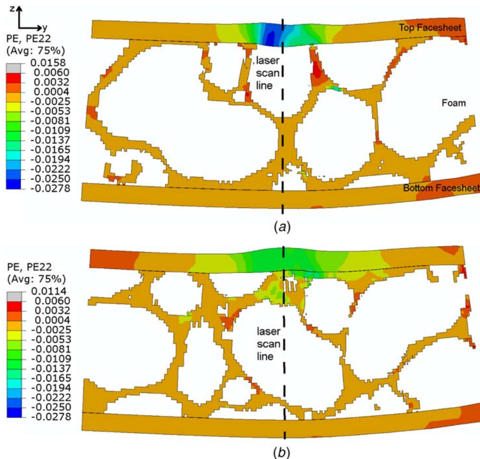
Fig. 14 Plastic strain distributions in the y -direction in a type II sandwich panel after a laser scan at a large spot size ( D = 12 mm, v = 10 mm/s), shown using a voxel model. The deformation was scaled by a factor of 10 for viewing clarity. The laser was scanned into the page, and the laser center was on the dashed line.
