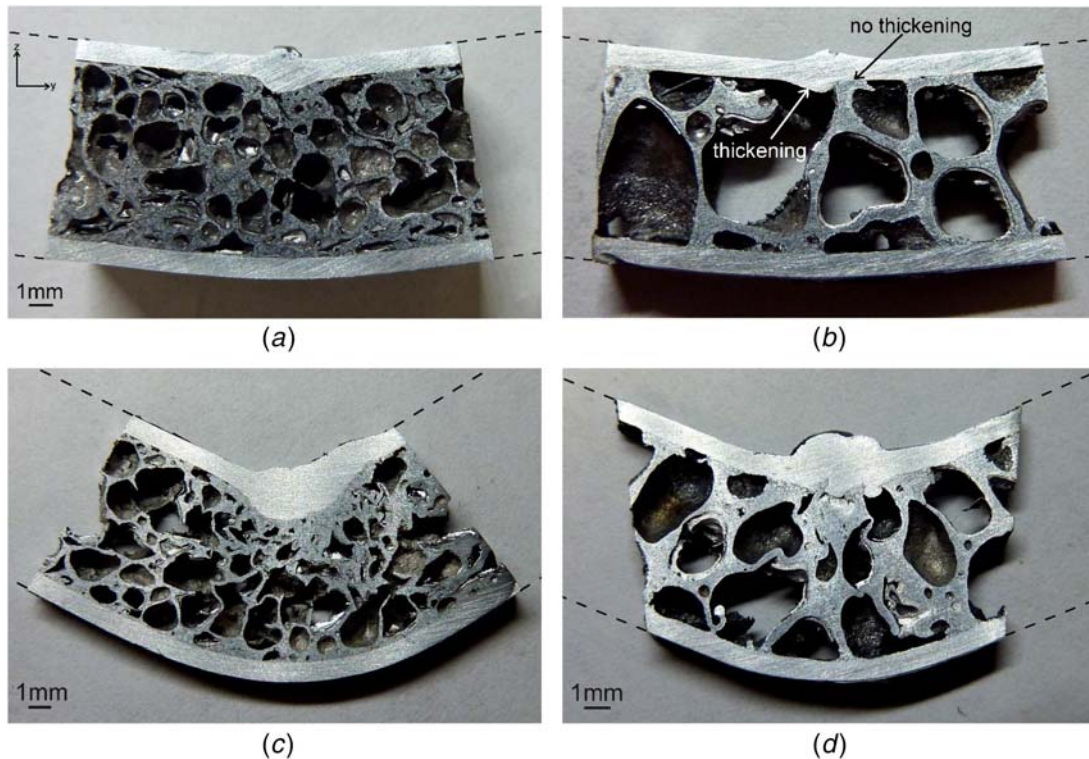
Fig. 13 Cross sections of type I and type II sandwich panels that were bent to the bending limit. The laser was scanned into the page. At a small spot size ( D = 4 mm, v = 30 mm/s), (a) the bending limit of the type I sandwich panel is around 15 deg and (b) for the type II sandwich panel it is around 12 deg (b). At a large spot size ( D = 12 mm, v = 10 mm/s), the limit is (c) around 65 deg for the type I sandwich panel, and (d) around 45 deg for the type II sandwich panel.
