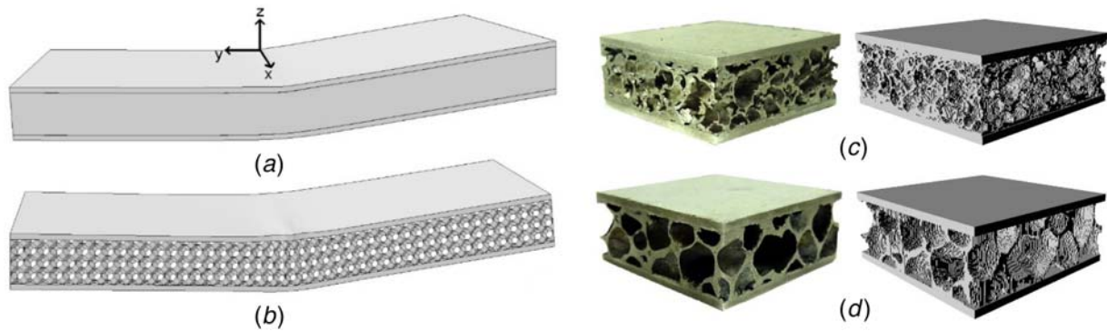
Fig. 4 (a) Equivalent sandwich model, (b) Kelvin-cell sandwich model, (c) type I sandwich panel specimen (left) and corresponding voxel model (right), and (d) type II sandwich panel specimen (left) and corresponding voxel model (right)
