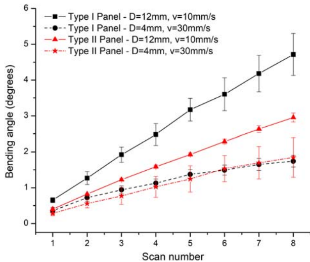
Fig. 5 Bending angles of both sandwich panel types over 8 laser scans at a large spot size ( D = 12 mm, v = 10 mm/s) and a small spot size ( D = 4 mm, v = 30 mm/s), the power was constant at P = 800 W. The results were averaged over three specimens; standard errors are shown.
