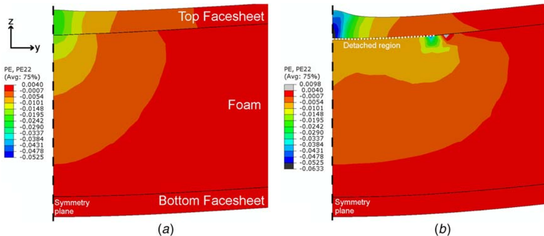
Fig. 17 Plastic strain distributions in the y -direction after a laser scan at a large spot size ( D = 12 mm, v = 10 mm/s). In (a), the adhesion between the top facesheet and the foam core is intact, whereas in (b), the top facesheet is detached from the foam core over a half the spot size of D = 12 mm. Only half of the model is shown due to symmetry. The deformation was scaled by a factor of 10 for viewing clarity.
