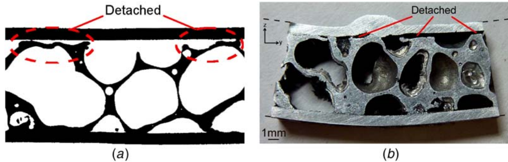
Fig. 16 (a) A cross section of the type II sandwich panel obtained using a micro-CT scan shows that there are regions of detachment between the facesheet and the foam core. This detachment is detrimental to laser forming since the maximum achievable bending angle drops from 45 deg to around 15 deg at a large spot size ( D = 12 mm, v = 10 mm/s), shown in (b).
