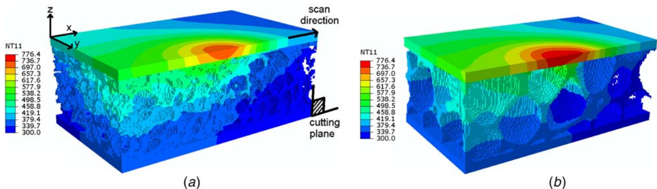
Fig. 12 Temperature distribution in voxel models of (a) type I sandwich panels and (b) type II sandwich panels, during a scan at a large spot size ( D = 12 mm, v = 10 mm/s). The laser was scanned in the x-direction. The models were sliced along the laser scan line for viewing clarity.
