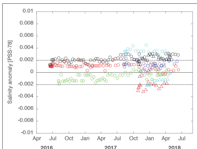
FIGURE 8 | Salinity difference between Deep SOLO SBE-61 CTDs and ship-based hydrographic data interpolated at Deep SOLO float location, projected on 0.74^{\circ}\text{C} potential temperature surface. CTD measurements are for 11 Deep SOLO floats deployed in the Southwest Pacific Basin (WMO ID numbers 5902456, 5902457, 5902478, 5902528, 5902529, 5905161, 5905162, 5905163, 5905164, 5905234, 5905235).
