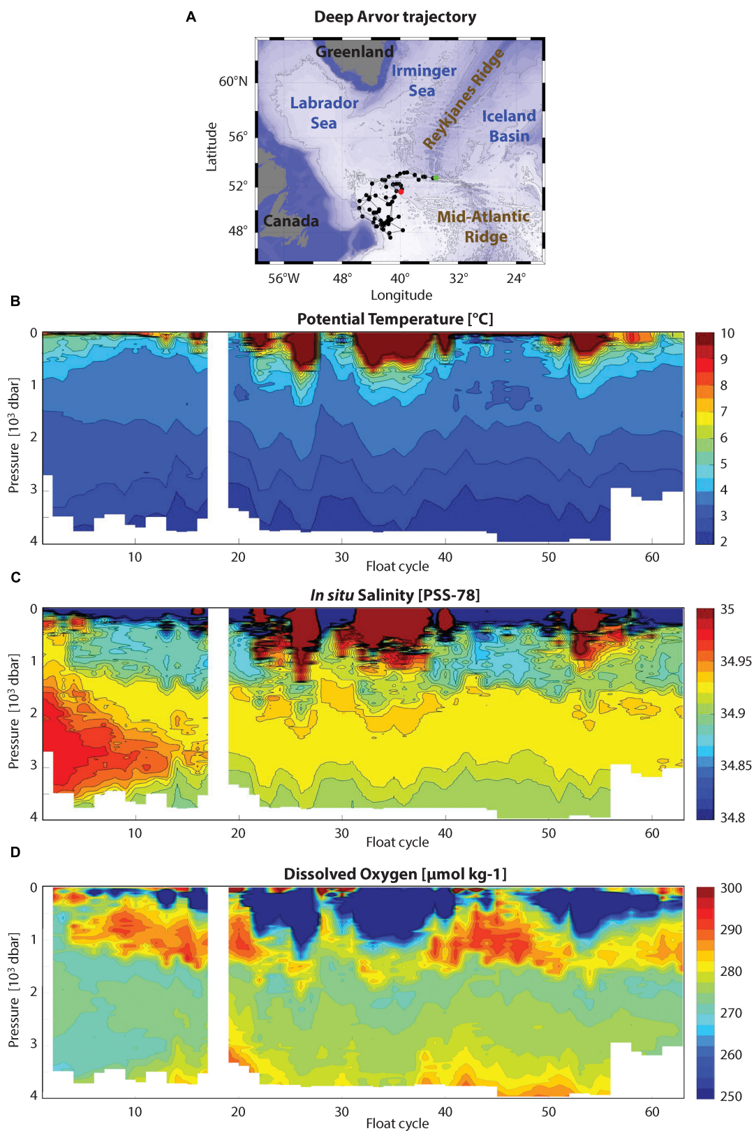
FIGURE 7 | (A) Trajectory of a Deep Arvor float (WMO ID 6901758) deployed in the North Atlantic Basin between July 2015 and March 2017. Locations of float deployment (rounded green symbol) and last observation (rounded red symbol) are indicated. (B) Potential temperature, (C) In situ salinity, and (D) Dissolved oxygen (DO) measurements from the Deep Arvor float between July 2015 and March 2017.
