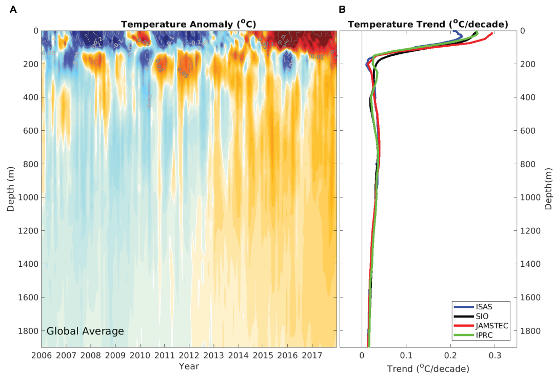
FIGURE 12 | (A) Global averaged temperature anomaly ( ^{\circ}\text{C} – from SIO) and (B) trend ( ^{\circ}\text{C}/\text{decade} , 2006–2018) versus depth, based on gridded Argo data. Gridded product sources are: ISAS (Gaillard et al., 2016), SIO (Roemmich and Gilson, 2009); IPRC- from the Asia-Pacific Data Research Center ( http://apdrc.soest.hawaii.edu/projects/Argo/data/gridded/On_standard_levels/index-1.html ); JAMSTEC (Hosoda et al., 2008).
