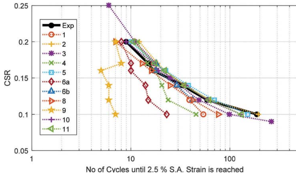
Figure 3. Comparison of the simulated liquefaction strength curves by different numerical simulations teams with the experimental results for e = 0.585 ( Dr \sim 71.5\% ).
