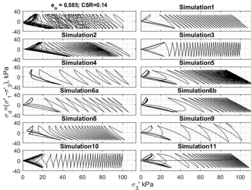
Figure 1-a. Comparison of the numerical simulations of stress paths for a cyclic stress-controlled test on Ottawa F65 sand. e = 0.585 ( Dr \sim 71.5\% ), p'_0 = 100 kPa, CSR = 0.14 .
