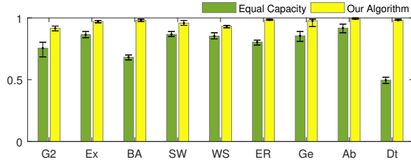
Fig. 2. Comparison of normalized caching gains for graphs in Table I.
