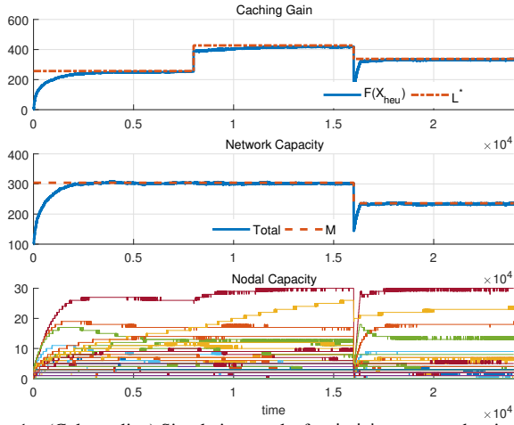
Fig. 1. (Color online) Simulation results for dtelekom network using cache allocation X_{heu} obtained from our heuristic placement in Sect. IV-D.2. L^* from (10) is obtained by a centralized algorithm and is an upper bound on the optimal caching gain. Bottom plot shows cache sizes c_v(t), \forall v \in \mathcal{V} .
