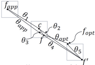
Figure 25: Illustration of \theta_{app} v.s. \theta_{opt}
