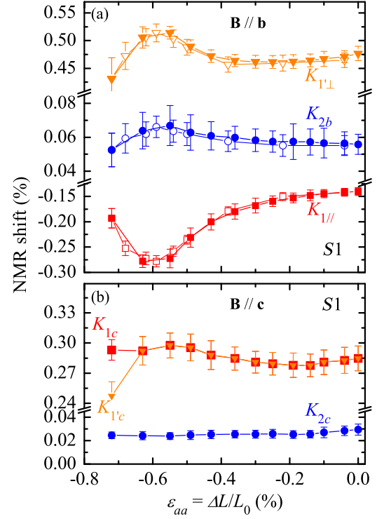
FIG. 4. Measured NMR shifts for \mathbf{B} \parallel \mathbf{b} (a) and for \mathbf{B} \parallel \mathbf{c} (b) at T = 4.3 K. The solid (open) symbols represent increasing (decreasing) |\epsilon_{aa}| . The error bars are determined by the half-width of the peaks. Similar results are reproduced from several samples; see Fig. S5(a) in the Supplemental Material [32].
