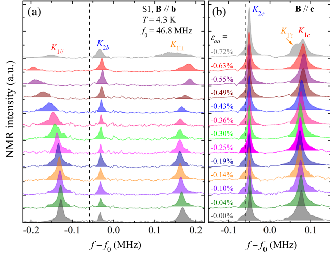
FIG. 3. NMR spectra of the central transitions ( \frac{1}{2} \leftrightarrow -\frac{1}{2} ) of O(1), O(1'), and O(2) at various strains for magnetic field along the \mathbf{b} (left) and \mathbf{c} axes (right). The measurements are carried out at fixed temperature ( T = 4.3 K) and field ( B = 8.0970 T) and radio frequency f_0 = 46.80 MHz. The curves are vertically offset for clarity. The dash vertical line corresponds to ^{17}\gamma = -5.7719 MHz/T ( \text{D}_2^{17}\text{O} ) [30] with zero shift.
