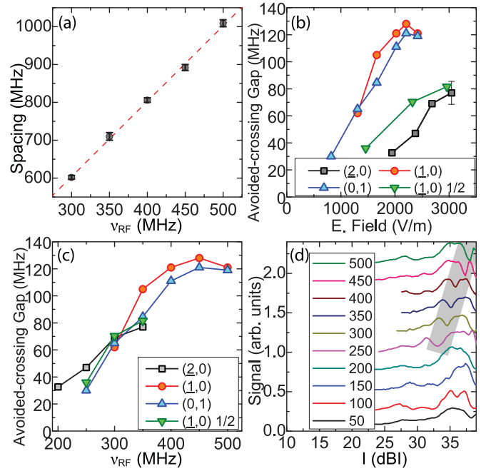
FIG. 5. Effect of applied rf frequency on 30D Rydberg levels. (a) Frequency separation between m_J = 3/2 (1, 0) and (0, 1) avoided-crossings versus rf frequency. A linear fit (dashed line) gives a slope of 1.99 \pm 0.05 ( r^2 = 0.997 ). (b) Measurement of the gap size versus applied electric field (V/m), for observed avoided crossings. All avoided crossings are of m_J = 3/2 , except for the inverted triangles ( m_J = 1/2 ). (c) Measurement of the avoided-crossing gap size versus applied rf frequency. (d) Change in probe beam transmission signal showing EIT versus intensity (dBI) at a fixed frequency of -100 MHz (relative to the 30D_{5/2} zero-field resonance), for various applied rf frequencies (MHz). The highlighted region shows the m_J = 3/2 (1, 0) avoided crossing shifted up in dBI for increasing rf frequency.
