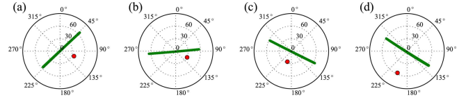
Figure 2. The polar plot for the solar direction (red dot) and the RSP scanning direction (green line) for each case listed in Table 1: (a) SABOR-Open, (b) SABOR-Coastal, (c) NAAMES-Open, and (d) NAAMES-Coastal. The north direction is chosen as azimuth angle zero.
