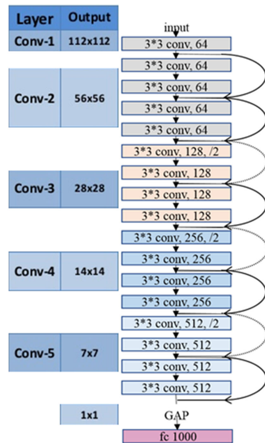
Fig. 4 Architecture of ResNet-18 [23]
