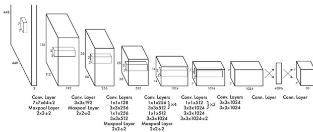
Fig. 3 24 convolutional layers followed by 2 fully connected layers for YOLO version 1 [21]
