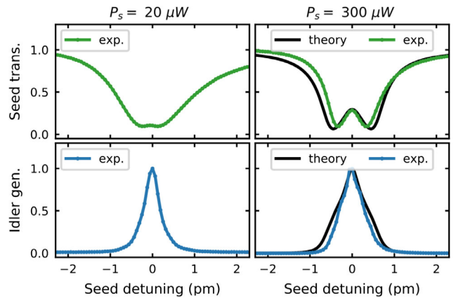
FIG. 4. Seed (green) transmission and idler (blue) generation when seed wavelength is scanned across the resonance. On the left, the seed power P_{\text{seed}} = 20 \mu\text{W} . On the right, where P_{\text{seed}} = 300 \mu\text{W} , the profiles are modified by the strong nonlinear coupling.
