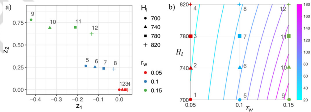
Figure 7. (a) estimated 2D mapped LVs representing the 12 levels of the qualitative factor t in the revised borehole example. The latent representation successfully uncovered the structural dependence of the factor levels on the two underlying numerical variables: the three levels of r_w (represented by colors) are distributed along z_2 dimension and within each r_w group the four levels of H_I correspond to z_1 varying; (b) contour plot of the response in revised borehole example as a function of r_w and H_I with the other numerical variables in Table S1 fixed at their mean values.
