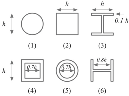
Figure 1. Six cross-sectional shapes, corresponding to six levels of the qualitative factor for the beam bending example: (1) circular cross-section with diameter h ; (2) square cross-section with height and width h ; (3) I-shaped cross-section with height and width h and thickness 0.1h ; (4) hollow square cross-section with outer side length h and thickness 0.15h ; (5) hollow circular cross-section with outer diameter h and thickness 0.15h ; (6) H-shape cross-section with height and width h and thickness 0.1h .
