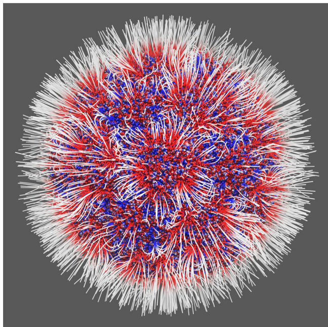
Figure 3. Electrostatic field lines human parainfluenza virus: red and blue correspond to negative and positive polarity, respectively. The modeling was done using PDB ID 5MJV, which contains 180 proteins, including 41,880 residues. The diameter of the whole virus is 298 Å.
