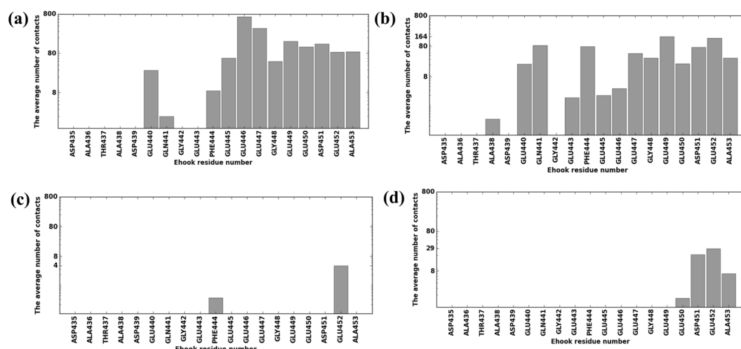
Figure 4. The MTBD made contacts primarily with the distal tip of E-hook D. Bars represent the average contacts made by each E-hook D residue (in logarithmic scale) and the MTBD at MTBD-microtubule distances of 0, 5, 15 and 25 Å (panels a–d, respectively). Three independent runs (see Methods) were analyzed and results averaged for each distance, and 2000 total frames were analyzed for each run.
