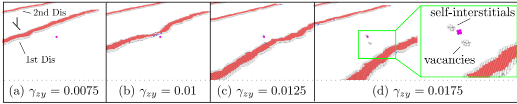
Figure 12: Snapshots of the first edge dislocation bypassing an impenetrable precipitate with D = 0.56 nm following the Hirsch looping mechanism. In (d), two self-interstitials and two vacancies are formed in the vicinity of the precipitate. Atoms on the precipitate surface are rendered in magenta.
