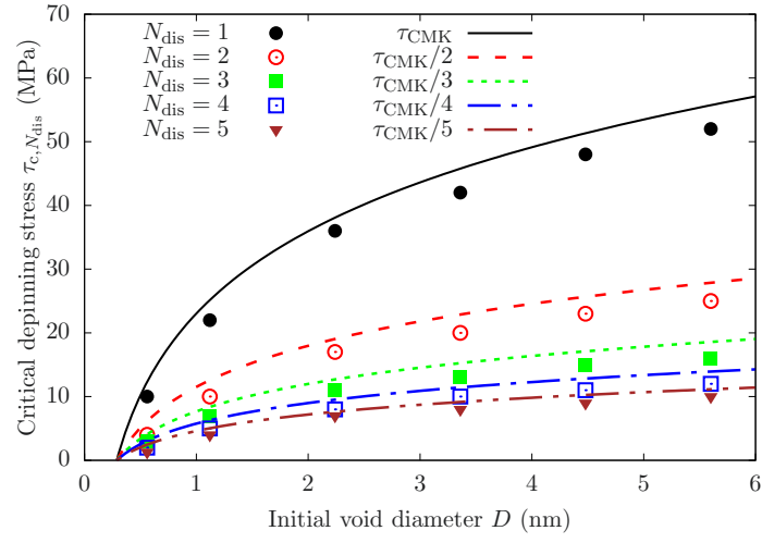
Figure 6: CAC-based depinning stress with respect to the initial void diameter D taken at the first dislocation exiting the void when N_{dis} varies from 1 to 5. The predictions by Eq. 13 are also shown.
