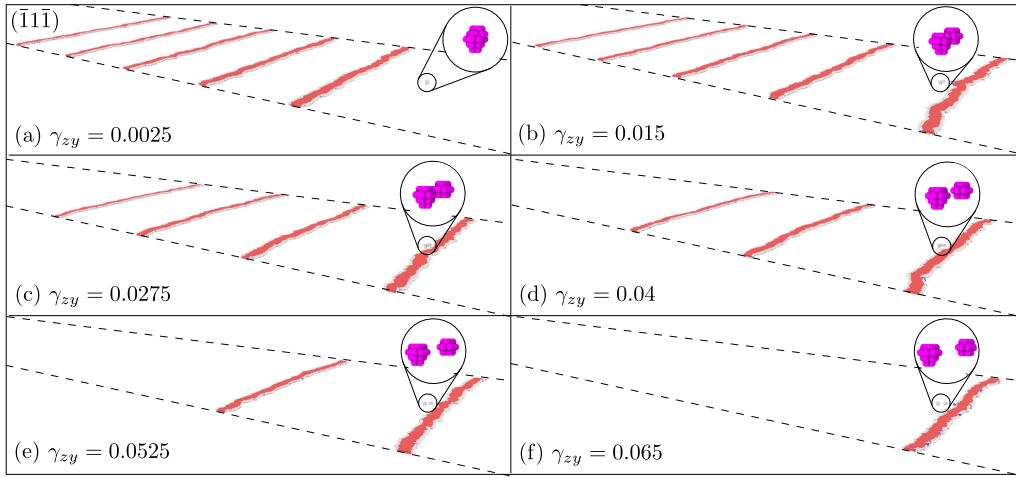
Figure 7: Snapshots of five edge dislocations sequentially bypassing a void with D = 0.56 nm. After bypassed by the second dislocation, shown in (c), the original spherical void, which contains seven vacancies, is split into two smaller hemispherical voids, with the left and right ones containing four and three vacancies, respectively. In the insets, atoms on the void surface are in magenta.
