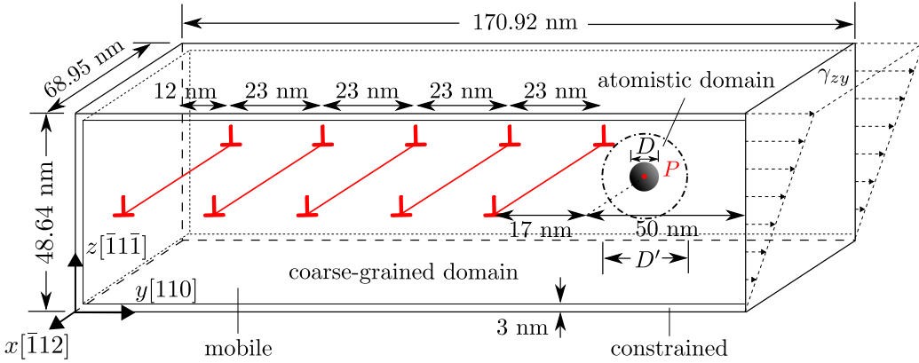
Figure 3: Illustration of the simulation cell for interactions between five edge dislocations in a planar array and an obstacle (filled black sphere centered at the red point P with diameter D ), which is either a void or an impenetrable precipitate. An atomistic domain is meshed within a sphere centered at P with diameter D' to let the obstacle deform and dislocations evolve at full atomic resolution, while the coarse-grained domain with 3D rhombohedral elements is employed elsewhere. Five initially equally spaced edge dislocations in the coarse-grained domain having the same Burgers vector \mathbf{b} = (a_0/2)[110] are placed on the same (\bar{1}1\bar{1}) slip plane. Note that (i) owing to the PBCs applied along the x direction, the dislocations are infinitely long and the obstacles form an infinitely long periodic array, and (ii) after energy minimization, the dislocations become dissociated and are no longer equally spaced along the y direction, as expected.
