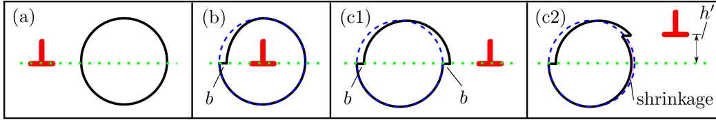
Figure 1: Illustrations of two edge dislocation/void interaction mechanisms, distinguished by whether or not the dislocation undergoes a climb process. The green dotted line is the original slip plane; the black solid and blue dashed circles are the current and original void shape, respectively. In both mechanisms, the dislocation creates two surface steps with magnitude b on the incoming and outgoing sides of the void, respectively. In (c1), the dislocation does not climb and the outgoing surface step forms on the original slip plane; in (c2), the dislocation climbs by h' with respect to the original slip plane by absorbing some vacancies from the void, leaving behind a surface step on the outgoing slip plane. In (c2), the void shrinks by the violet area (denoted “shrinkage”). Note that in 3D, a jog is formed on the dislocation line in (c2).
