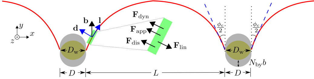
Figure 4: Illustration of the critical dislocation depinning configuration when the dislocation is about to exit a void. Projected on the slip plane, two hemispheres of the original spherical void with initial diameter D are shifted against each other by N_{by}b after N_{by} dislocation bypasses; the yellow shaded lenticular region is the overlapped section between the two hemispheres. \mathbf{b} is the Burgers vector of the dislocation, \mathbf{l} is the unit vector along the dislocation line, \mathbf{d}(\perp \mathbf{l}) is the unit vector along the dislocation moving direction, L is the intervoid ligament distance, D is the initial void diameter, and \phi_c is the depinning angle.
