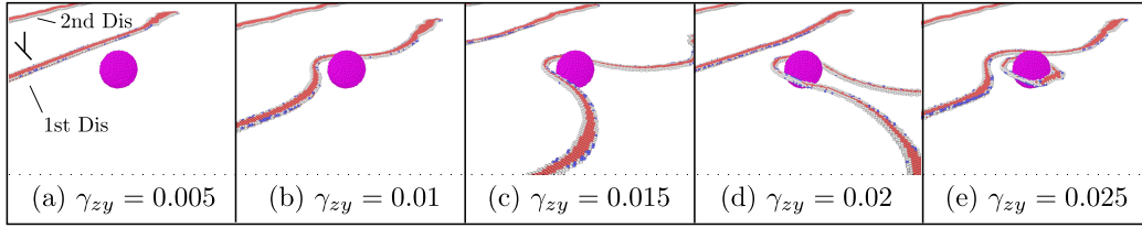
Figure 10: Snapshots of the first edge dislocation bypassing an impenetrable precipitate with D = 5.6 nm following the Orowan looping mechanism. In (b–d), the dislocation bows around the precipitate; in (e), the dislocation glides away with a shear loop left behind. Atoms on the precipitate surface are rendered in magenta.
