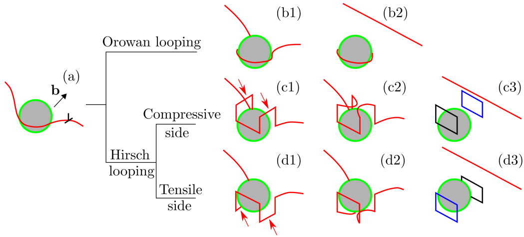
Figure 2: Illustrations of two dislocation/impenetrable precipitate interaction mechanisms: Orowan looping and Hirsch looping. Other mechanisms may apply if the precipitate is too small. In (a), the red curve is the edge dislocation, with its extra half-plane above the slip plane. Hence, the compressive and tensile sides of the dislocation stress field lie above and below the slip plane, respectively. In Orowan looping, the dislocation bows around the precipitate in (b1) and a shear loop is left behind in (b2). In Hirsch looping, the screw components (red arrows) of the dislocation cross slip toward the (c1) compressive or (d1) tensile side of the original slip plane; in (c2) and (d2), the two screw dislocation segments with the same Burgers vector but opposite line directions move together to annihilate each other; in (c3) and (d3), edge prismatic loops of interstitial (in black) and vacancy (in blue) types are formed. Note that (b1) and (b2) hold for dislocations with any character angle in Orowan looping, while the illustrated Hirsch looping mechanism only applies to edge dislocations.
