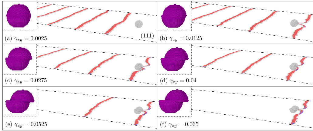
Figure 8: Snapshots of five edge dislocations sequentially bypassing a void with D = 5.6 nm. After each dislocation bypass, two steps are created on the surface of the void. In the insets, atoms on the void surface are in magenta.
