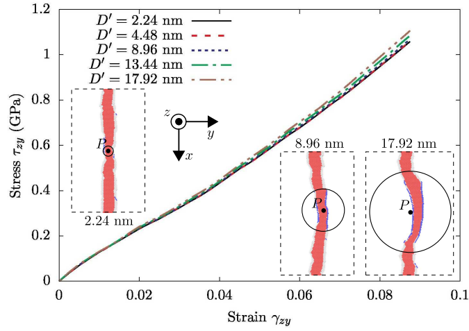
Figure A2: Stress-strain curves of the simulation cells containing an array of five pre-existing dislocations but no obstacle. In each case, an atomistic domain is resolved within the sphere centered at P with diameter D' . The curves for different D' are close to each other. The three insets, which show the first edge dislocation configurations at \gamma_{zy} = 0.01 , are for D' = 2.24 , 8.96, and 17.92 nm, respectively. The view is illustrated by the coordinate system. The extended dislocation is found to have a smaller stacking fault width in the atomistic domain than in the coarse-grained domain, as expected [37].
