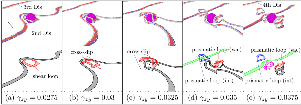
Figure 11: Snapshots of the second edge dislocation bypassing an impenetrable precipitate with D = 5.6 nm following the Hirsch looping mechanism. In the first row, atoms on the precipitate surface are rendered in magenta. In the second row, different dislocations are distinguished by colors.
