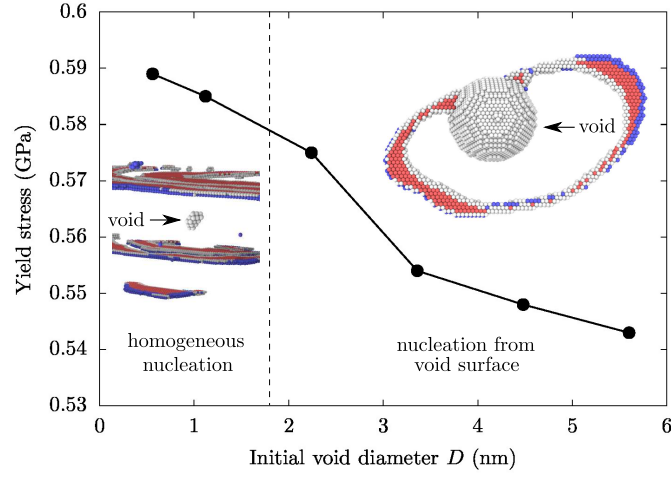
Figure A1: Yield stress with respect to the initial void diameter D for simulation cells containing a void but no pre-existing dislocation. When D = 0.56 and 1.12 nm, dislocations are nucleated homogeneously in the material; for larger D , dislocations are nucleated from the void surface. The two insets are for D = 0.56 and 5.6 nm, taken on the threshold of plasticity at \gamma_{zy} = 0.12 and 0.102 , respectively.
