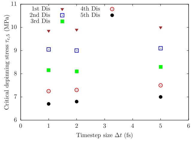
Figure B1: CAC-based depinning stress as a function of the timestep size \Delta t at each dislocation exiting the void when N_{\text{dis}} = 5 and D = 5.6 nm.
