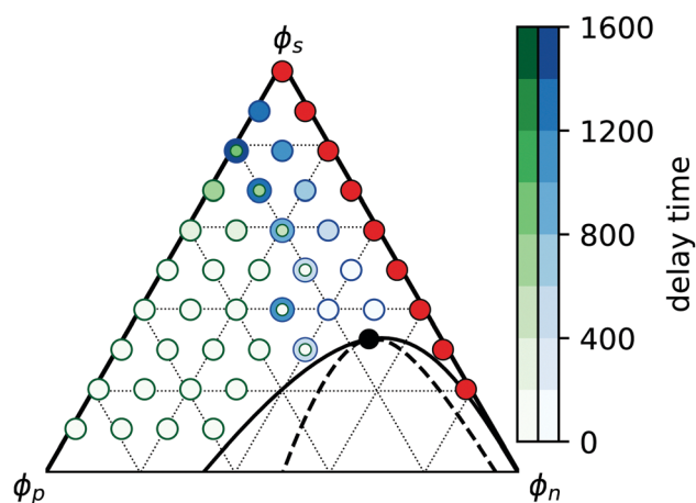
Fig. 9 Characterization of the late-time phase separation behavior according to the initial film composition. Red circles indicate no phase separation (regime I). Green circles indicate simple phase separation (regime II), where the shade of green denotes the delay time before the onset of phase separation. Blue circles indicate spinodal decomposition (regime III), where the shade of blue denotes the delay time. As indicated, some film compositions in the middle of the phase diagram transition between regimes II and III.
