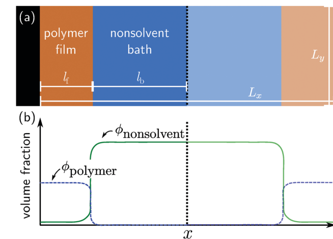
Fig. 2 (a) A 2D representation of the simulation geometry for a polymer film of thickness l_f and bath height l_b . With periodic boundary conditions, one employs an initial condition that is symmetric about the dashed center-line and l_b \gg l_f . For non-periodic boundary conditions where the bath composition is known, no such requirements are necessary, but different methods must be used to discretize space. (b) A 1D plot showing example polymer and non-solvent volume fractions in both film and bath domains corresponding to the 2D schematic in panel (a).
