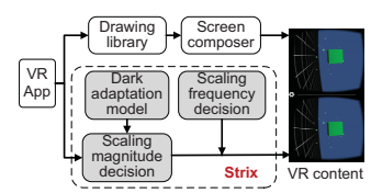
Figure 2: Architecture of Strix.
