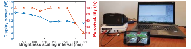
Figure 7: Scaling frequency impacts both power and experience.
