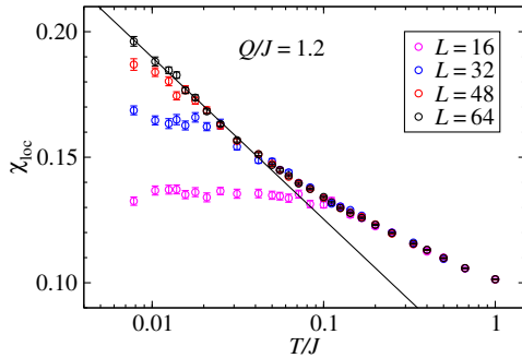
FIG. 20. Temperature dependence of the local susceptibility of the random- Q model at its AFM-RS transition for several different system sizes. The line is a fit of the L = 64 low- T points to the logarithmically divergent form in Eq. (18).
