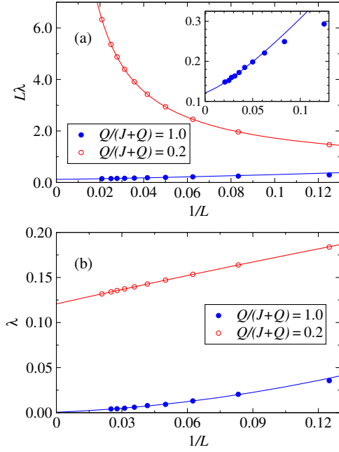
FIG. 10. Finite-size scaling properties of the string fraction \lambda of the random- Q model in the AFM state at Q/(J+Q) = 0.2 and deep in the RS phase at Q/(J+Q) = 1.0 . In (a), \lambda is scaled by L to demonstrate \lambda \propto L^{-1} in the RS phase (the inset shows the results on a more detailed scale). The results in (b) illustrate the expected size-independent string fraction in the AFM phase. Error bars are smaller than the symbols.
