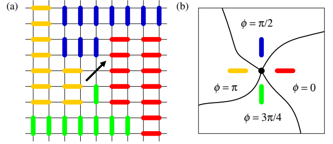
FIG. 3. (a) Illustration of a spinon forming at an unpaired spin at the nexus of domain walls separating the four different columnar VBS patterns on the square lattice. (b) The four VBS patterns associated with angles \phi in a simplified view of the VBS vortex, with only the bonds closest to the core shown in the same color coding as in (a). A similar vortex can also be constructed starting from core bonds rotated by 90^\circ relative to those shown here.
