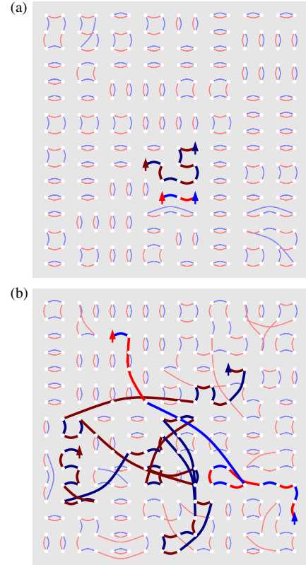
FIG. 6. Transition graphs in the S = 1 ground state of an L = 16 J - Q system without disorder in the VBS (a) and AFM (b) phase. For clarity, open boundaries are used here to avoid bonds crossing the boundaries. Red and blue arches correspond to bra and ket valence bonds, with thicker bonds representing the two open strings (depicted in different color shades for clarity) that terminate at unpaired spins (one in the bra and one in the ket state). These end spins are always on sublattice A in one of the strings and B in the other one. In (a), defects in the columnar symmetry-broken VBS pattern originate both from the presence of the spinons and by the intrinsic VBS fluctuations. Formation of a clearly columnar state can be observed only for much larger system sizes [55].
