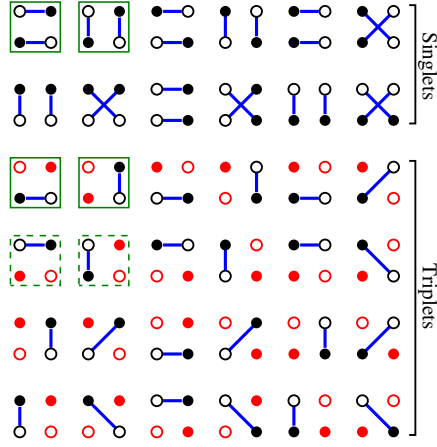
FIG. 28. Spinon wave-function components for singlet and triplets of two spinons and two antispinons, with the circles in order \frac{1}{2} \frac{3}{4} corresponding to the bright (spinon) regions in Fig. 26. Spinons (on sublattice A ) and antispinons (on sublattice B ) are denoted by solid and open circles, respectively, and singlet pairs are indicated by lines connecting circles. Unpaired red circles correspond to up spins (or other triplet states of the pairs). The components enclosed by solid green squares represent the dominant components of the wave functions as discussed in connection with Fig. 27, and the dashed green boxes indicate further regular components in the triplet sector. All other configurations correspond to cross terms existing when spinons and antispinons can trade places.
