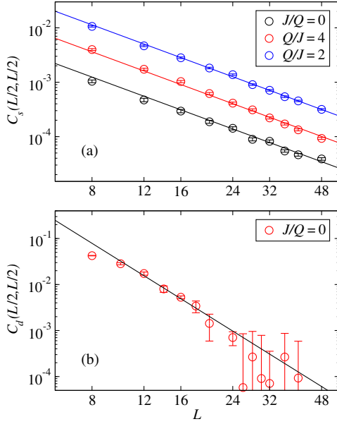
FIG. 12. Absolute values of the mean long-distance spin (a) and dimer (b) correlations at three coupling ratios inside the RS phase of the random- Q model. Results are shown at the largest distance on the periodic L \times L lattices. The three lines in (a) correspond to decay of the form \propto L^{-2} , and the line in (b) shows the form \propto L^{-4} .
