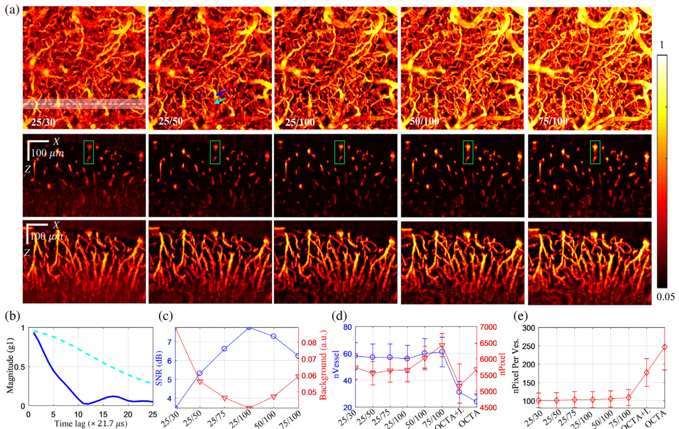
Fig. 5 (a) Comparison of g_1 -OCTA that obtained with different pairs of n_r/n_t ; top: en face MIP over a depth range of 400\ \mu\text{m} ; middle: single-XZ plane was obtained at the location marked by the dashed white line in en face MIP; bottom: XZ stack MIP was obtained from the white color-shaded region along Y; the two vessels marked by green rectangle were selected for quantitative analysis in Fig. 6; (b) |g_1(\tau)| obtained at a penetrating vessel (solid dark blue) and a transverse vessel (dashed light blue) marked by arrows in the en face MIP of 25/50 in (a); (c) SNR and average background noise for different g_1 -OCTA calculation pairs; (d) number of vessel cross sections averaged across all XZ planes and total number of pixels occupied by these vessel cross sections, OCTA+I.: OCTA obtained with Intralipid enhanced, OCTA: OCTA with intrinsic contrast (RBCs); and (e) averaged number of pixels per vessel cross section. Error bar: standard deviation, n = 400 (B-scans).
