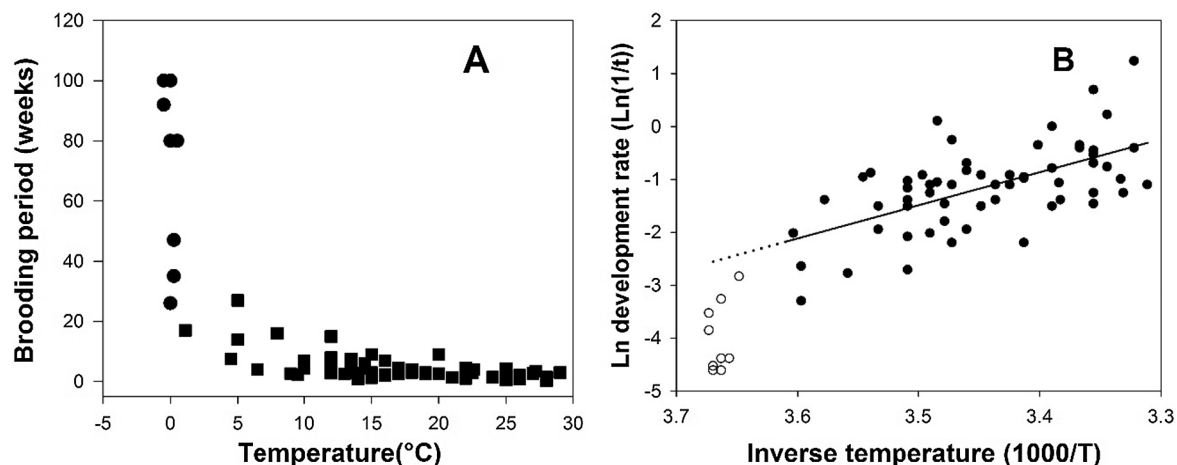
Fig. 12. Brooding period and development rates of brooding marine gastropod snails at ambient temperatures for tropical to polar species. (a) Time from brood initiation to release ( 1/\text{development rate} ) versus ambient temperature. In most cases, release is of crawling juveniles, but for two Antarctic species, release is of veliger larvae and development time to juvenile is approximately double that of brooding per se (Peck et al., 2006b). Data for 68 gastropod species, nine of which live at temperatures around 0 °C, show the full development period to juvenile. (b) Arrhenius plot of Ln developmental rate to juvenile stage for brooding gastropod molluscs. Fitted line is for temperate and tropical species (filled circles); brooding rate ( 1/\text{weeks} ) = 20.37 - 6.25 \times 1000/T ; r^2 = 0.36 , F = 32.4 , 58 df, p < 0.001 ; Antarctic species fall significantly below. Reproduced from Peck (2018).
