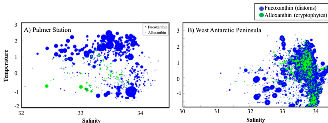
Fig. 5. The relative presence of diatoms (from fucoxanthin, blue) and cryptophytes (from alloxanthin, green) plotted in temperature-salinity phase space for (a) Palmer stations B and E, and (b) the Palmer LTER grid. The size of the circles indicates the relative concentration of chlorophyll a for discrete samples. Modified from Schofield et al. (2017). (For interpretation of the references to colour in this figure legend, the reader is referred to the web version of this article.)
