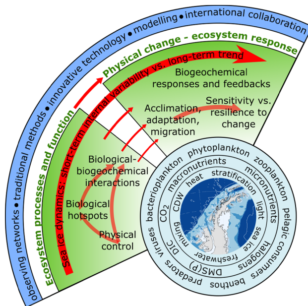
Fig. 3. Infographic summarising the key components of the WAP marine system, the most important mechanisms and interactions in the context of the two overarching questions addressed in this paper, and the major priorities and approaches for future marine research at the WAP.
