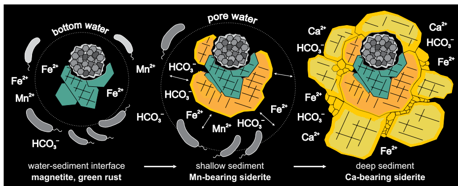
Figure 3. Sketch depicting growth of siderite after carbonate green rust and nano-magnetite. Diagenetic reduction of \text{Mn}^{4+} and \text{Fe}^{3+} and organic matter degradation lead to pore-water saturation with respect to siderite, initially forming Mn-bearing siderites. As pore water remains saturated with respect to siderite in the entire sediment sequence, siderite crystals continue to grow with depth into Ca-bearing mosaic monocrystals forming twins, bundles, and spheroidal aggregates.
