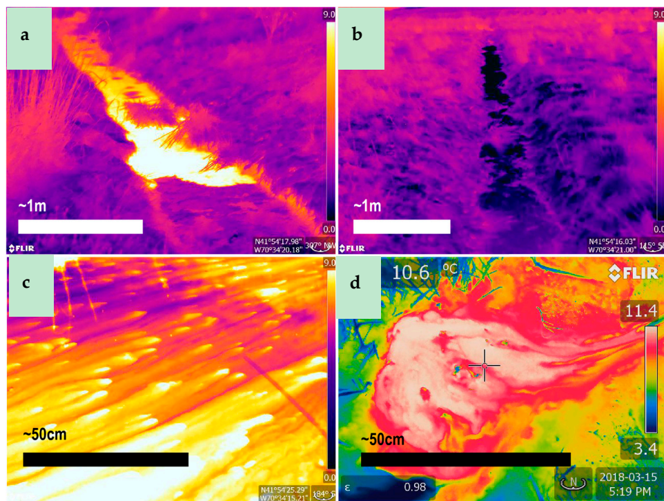
Figure 2. Hand-held thermal infrared (TIR) images collected before the restoration [16], along the relic cranberry peatland drainage ditches. Images show (a) natural groundwater discharge, (b) no discharge, (c) clustered centimeter-scale macropore discharge features, and (d) discrete discharge features observed after the restoration (March 2018) in similar locations to the pre-restoration period, indicating persistent subsurface hydrogeologic controls.
